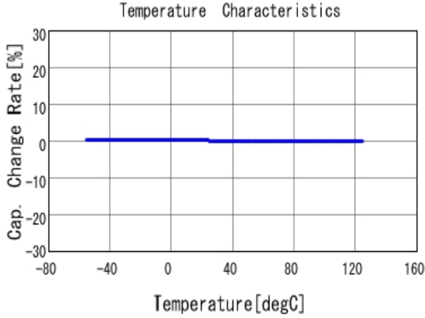
■ GRM1885C1H100JA01 C-Temp. capchange, DCOV, AC1Vrms
