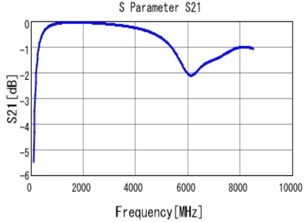
■ GRM1885C1H100JA01 S21 DCOV, 25degC
