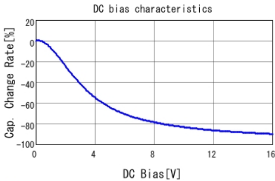
■ GRM185R61C475ME11 C-DC bias capchange, 25.0degC, AC1V
