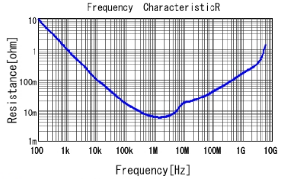
■ GRM185R61C475ME11 R DCOV, 25degC
