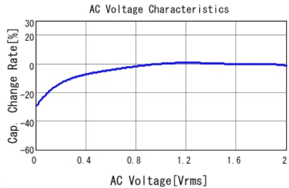
■ GRM185R61C475ME11 C-AC Voltage capchange, DCOV, 25.0d
