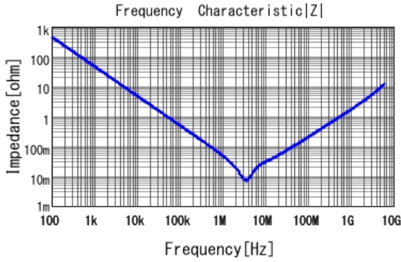
■ GRM185R61C475ME11 |Z| DCOV, 25degC
