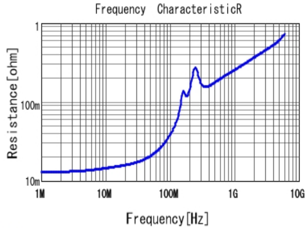
■ GRM1857U1A103JA44 R DCOV, 25degC
