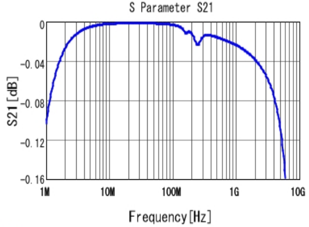
■ GRM1857U1A103JA44 S21 DCOV, 25degC
