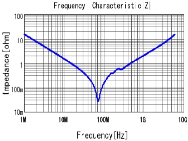
■ GRM1857U1A103JA44 |Z| DCOV, 25degC
