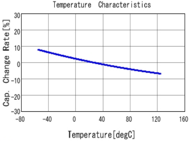
■ GRM1857U1A103JA44 C-Temp. capchange, DCOV, AC1Vrms
