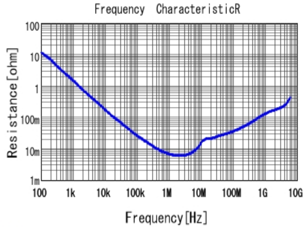
■ GRM155Z71A225KE44 R DCOV, 25degC
