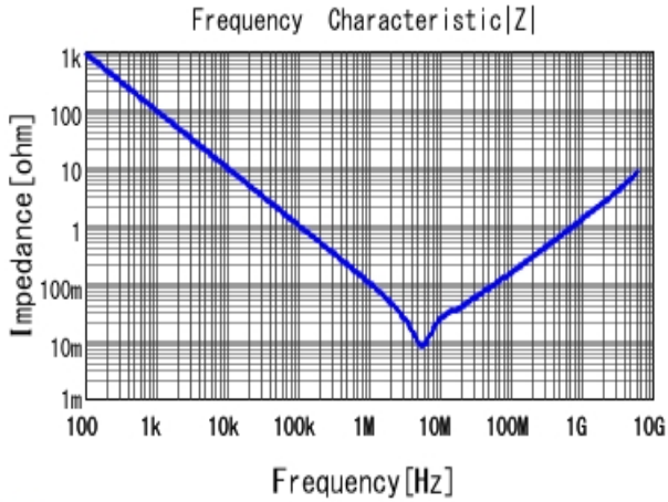
■ GRM155Z71A225KE44 |Z| DCOV, 25degC
