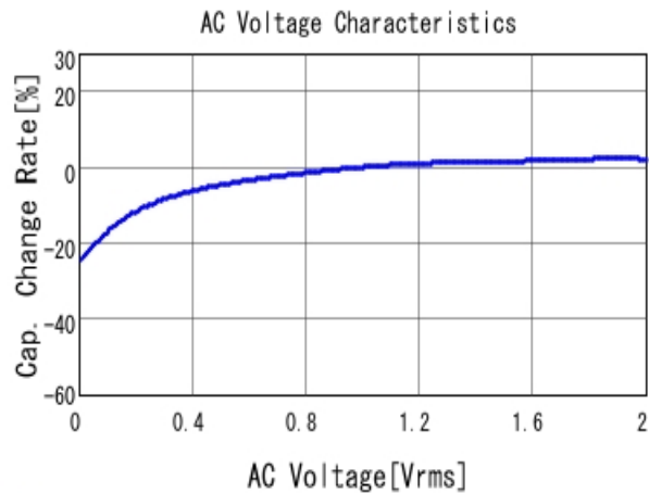
■ GRM155Z71A225KE44 C-AC Voltage capchange, DCOV, 25.0d
