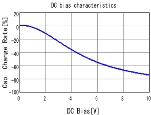
■ GRM155Z71A225KE44 C-DC bias capchange, 25.0degC, AC1V
