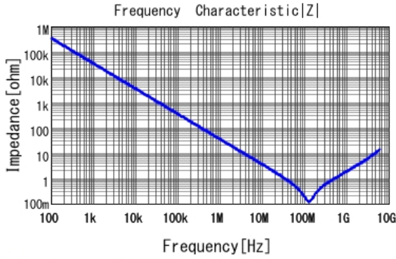
■ GRM155R72A472KA01 |Z| DCOV, 25degC
