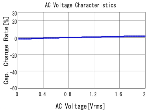
■ GRM155R72A471KA01 C-AC Voltage capchange, DCOV, 25.0d
