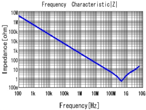
■ GRM155R72A471KA01 |Z| DCOV, 25degC
