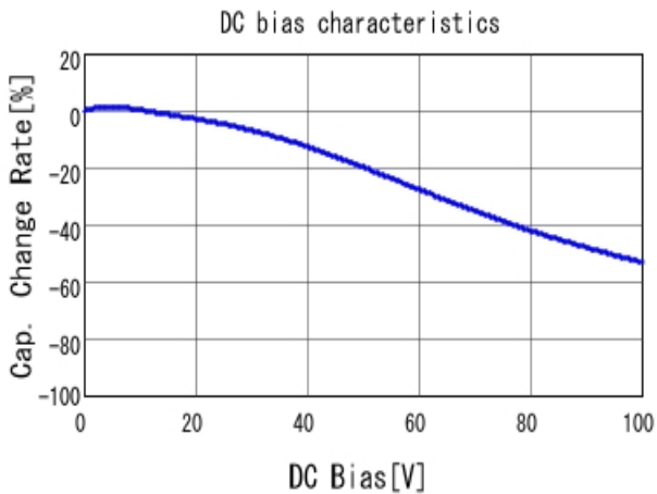
■ GRM155R72A471KA01 C-DC bias capchange, 25.0degC, AC1.
