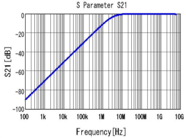
■ GRM155R72A471KA01 S21 DCOV, 25degC
