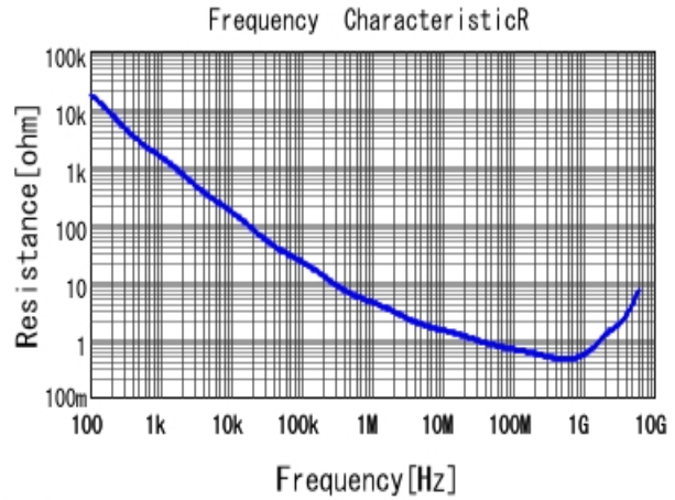
■ GRM155R72A471KA01 R DCOV, 25degC
