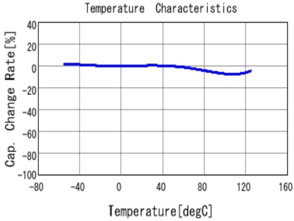
■ GRM155R72A471KA01 C-Temp. capchange, DCO. 0V, AC1.0Vrm
