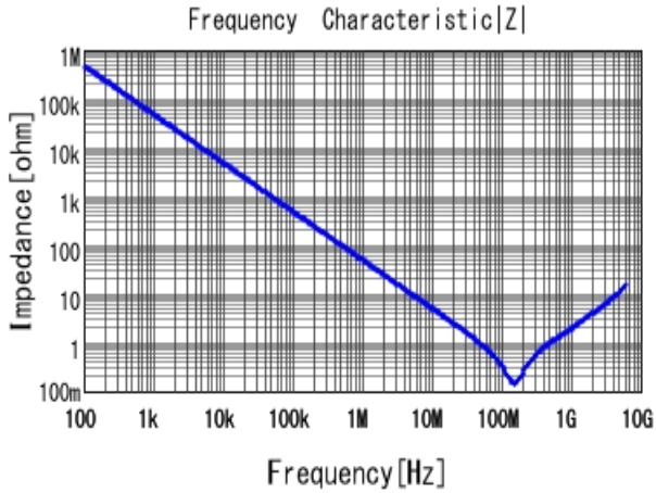
■ GRM155R72A332KA01 |Z| DCOV, 25degC
