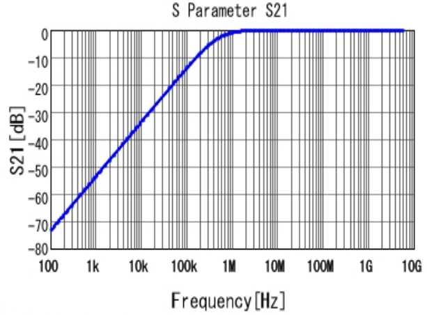
■ GRM155R72A332KA01 S21 DCOV, 25degC
