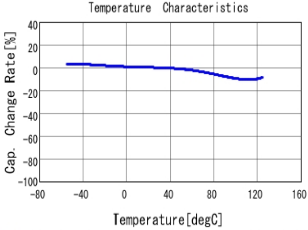
■ GRM155R72A332KA01 C-Temp. capchange, DCO. 0V, AC1.0V rm
