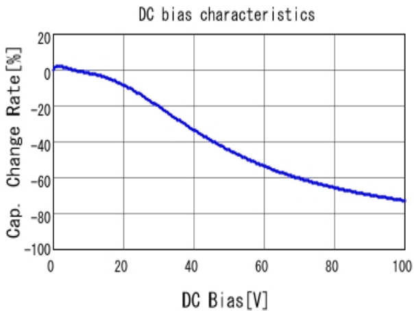
■ GRM155R72A332KA01 C-DC bias capchange, 25.0degC, AC1.
