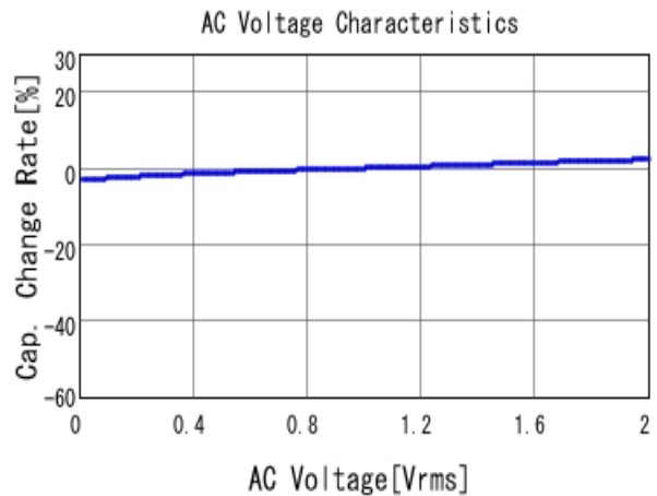
■ GRM155R72A332KA01 C-AC Voltage capchange, DCOV, 25.0d
