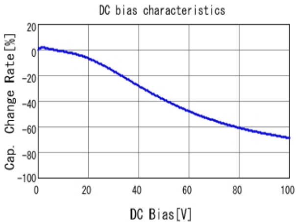
■ GRM155R72A102KA01 C-DC bias capchange, 25.0degC, AC1.
