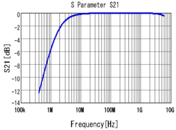
■ GRM155R72A102KA01 S21 DC0V, 25degC
