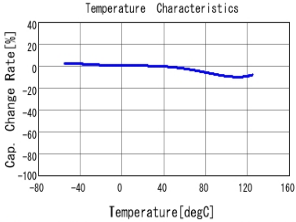
■ GRM155R72A102KA01 C-Temp. capchange, DC0.0V, AC1.0V rm
