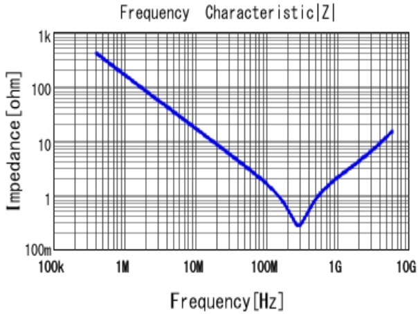
■ GRM155R72A102KA01 |Z| DCOV, 25degC
