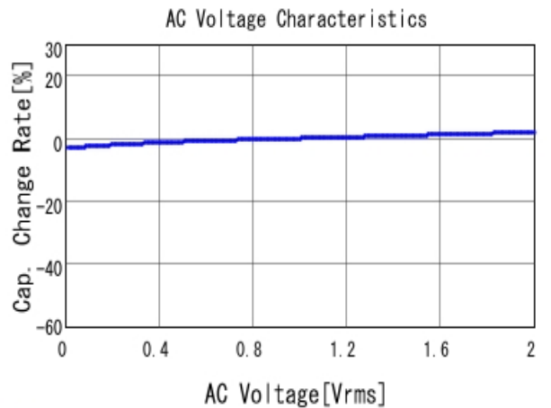
■ GRM155R72A102KA01 C-AC Voltage capchange, DCOV, 25.0d
