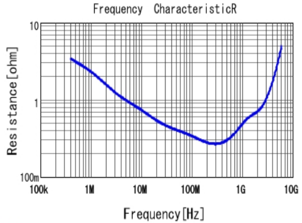
■ GRM155R72A102KA01 R DCOV, 25degC
