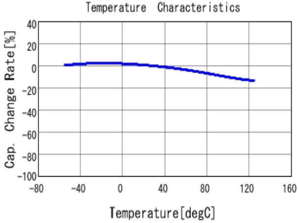
■ GRM155R71H683KE14 C-Temp. capchange, DCO. 0V, AC1.0V rm
