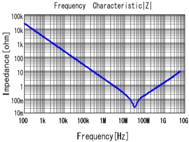
■ GRM155R71H683KE14 |Z| DCOV, 25degC
