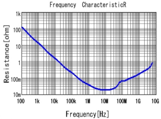
■ GRM155R71H683KE14 R DCOV, 25degC
