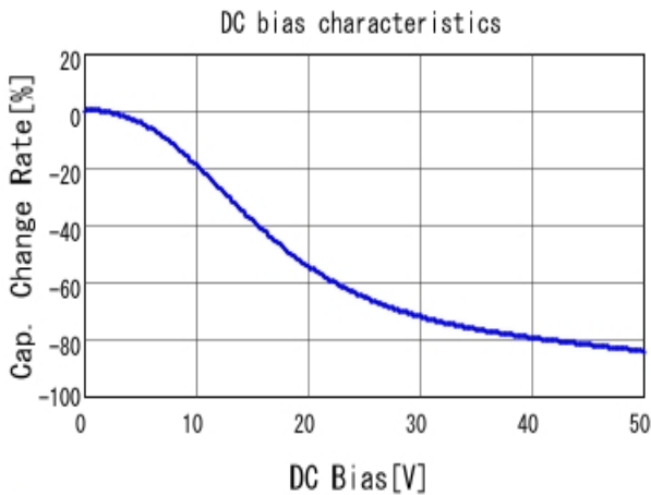
■ GRM155R71H683KE14 C-DC bias capchange, 25.0degC, AC1.
