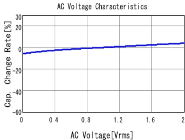
■ GRM155R71H683KE14 C-AC Voltage capchange, DCOV, 25.0d
