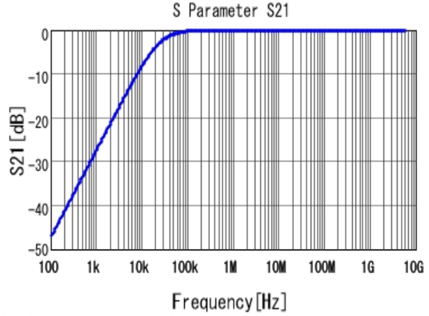
■ GRM155R71H683KE14 S21 DCOV, 25degC
