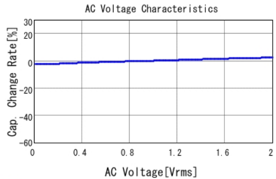
■ GRM155R71H682KA88 C-AC Voltage capchange, DCOV, 25.0d
