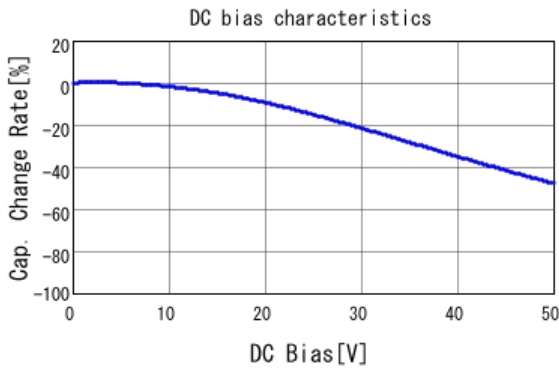
■ GRM155R71H682KA88 C-DC bias capchange, 25.0degC, AC1.
