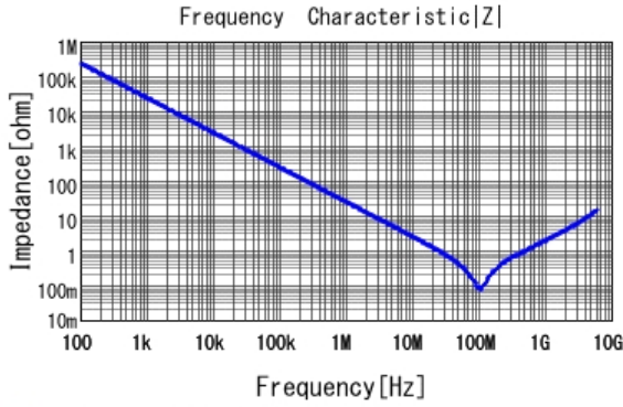
■ GRM155R71H682KA88 |Z| DCOV, 25degC
