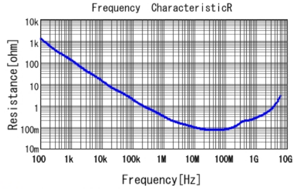
■ GRM155R71H682KA88 R DCOV, 25degC
