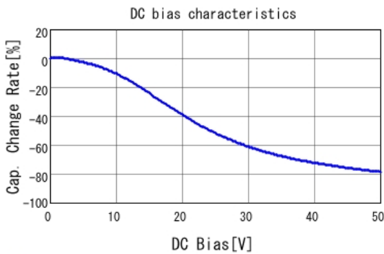
■ GRM155R71H473KE14 C-DC bias capchange, 25.0degC, AC1.
