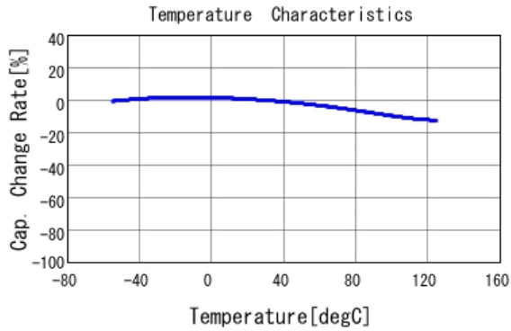
■ GRM155R71H473KE14 C-Temp. capchange, DC0.0V, AC1.0V rm
