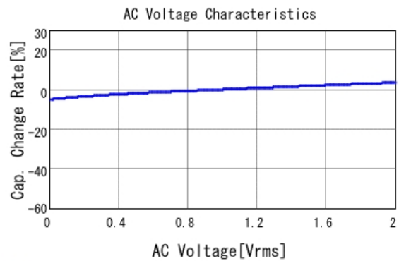
■ GRM155R71H473KE14 C-AC Voltage capchange, DCOV, 25.0d
