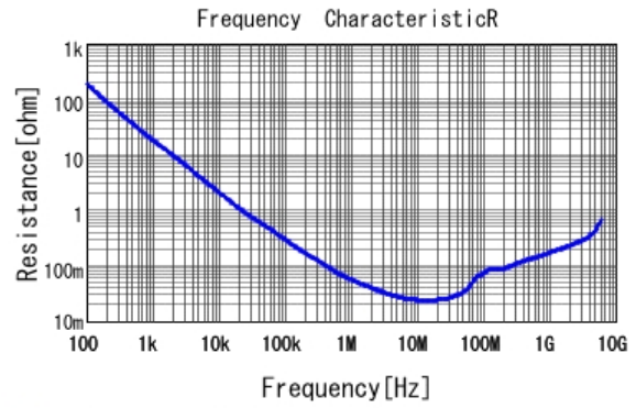
■ GRM155R71H473KE14 R DCOV, 25degC
