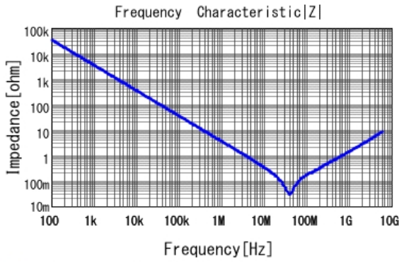
■ GRM155R71H473KE14 |Z| DCOV, 25degC
