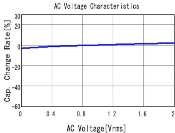
■ GRM155R71H472KA01 C-AC Voltage capchange, DCOV, 25.0d
