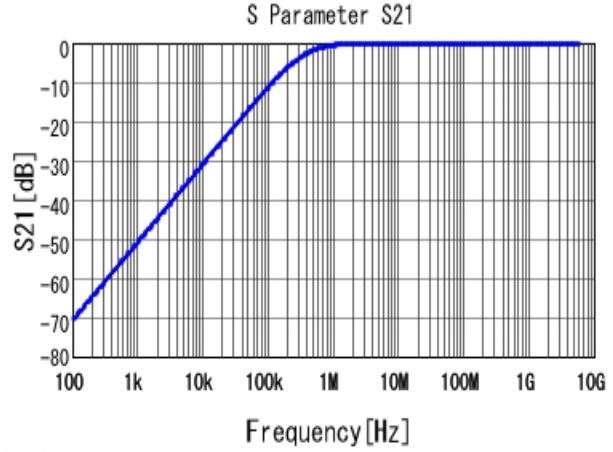
■ GRM155R71H472KA01 S21 DCOV, 25degC
