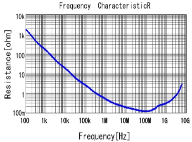
■ GRM155R71H472KA01 R DCOV, 25degC
