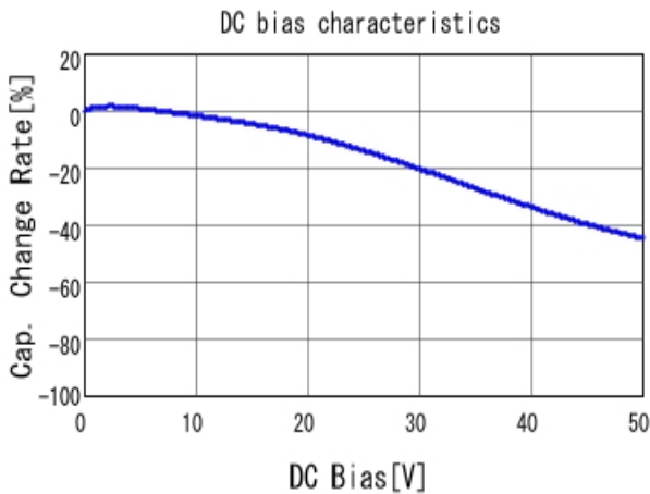
■ GRM155R71H472KA01 C-DC bias capchange, 25.0degC, AC1.
