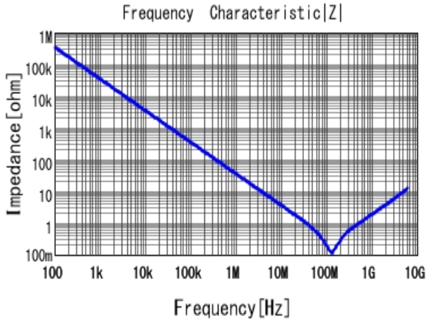
■ GRM155R71H472KA01 |Z| DCOV, 25degC
