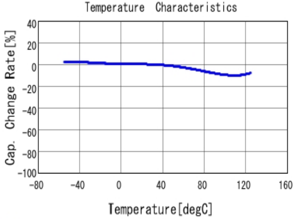
■ GRM155R71H472KA01 C-Temp. capchange, DCO. 0V, AC1.0Vrm
