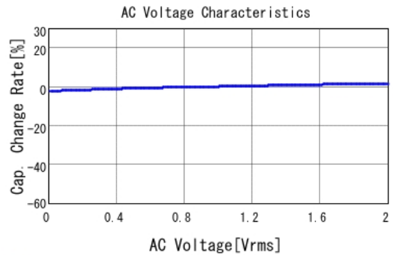
■ GRM155R71H471KA01 C-AC Voltage capchange, DCOV, 25.0d
