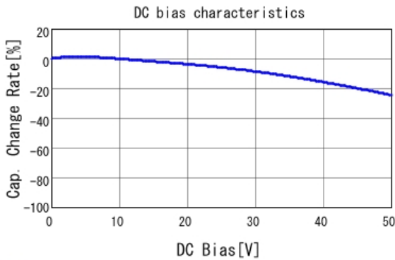
■ GRM155R71H471KA01 C-DC bias capchange, 25.0degC, AC1.
