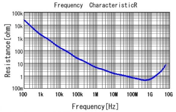
■ GRM155R71H471KA01 R DCOV, 25degC
