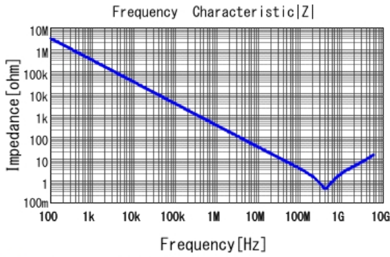
■ GRM155R71H471KA01 |Z| DCOV, 25degC
