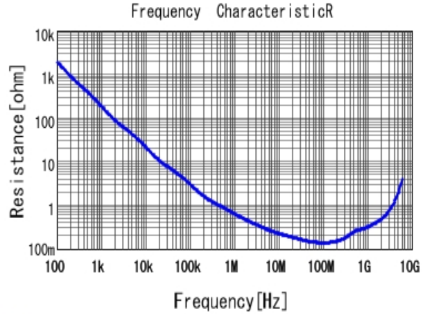
■ GRM155R71H392KA01 R DCOV, 25degC
