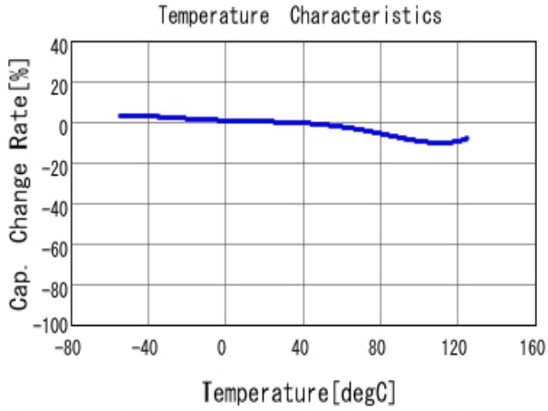
■ GRM155R71H392KA01 C-Temp. capchange, DCO. 0V, AC1.0Vrm
