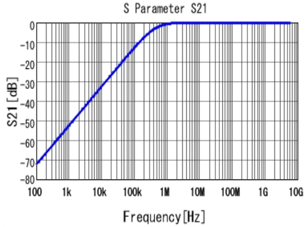
■ GRM155R71H392KA01 S21 DCOV, 25degC
