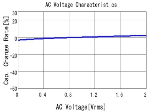
■ GRM155R71H392KA01 C-AC Voltage capchange, DCOV, 25.0d
