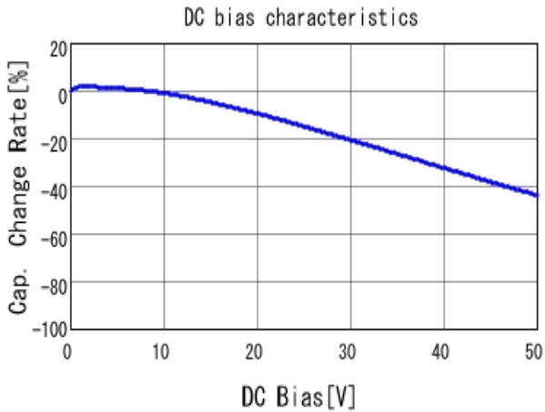
■ GRM155R71H392KA01 C-DC bias capchange, 25.0degC, AC1.
