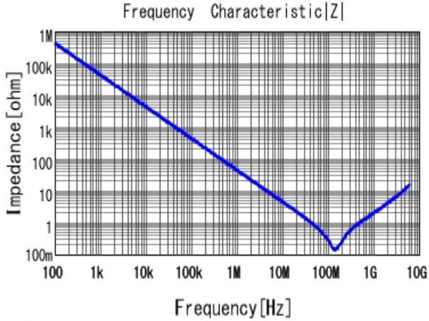
■ GRM155R71H392KA01 |Z| DCOV, 25degC
