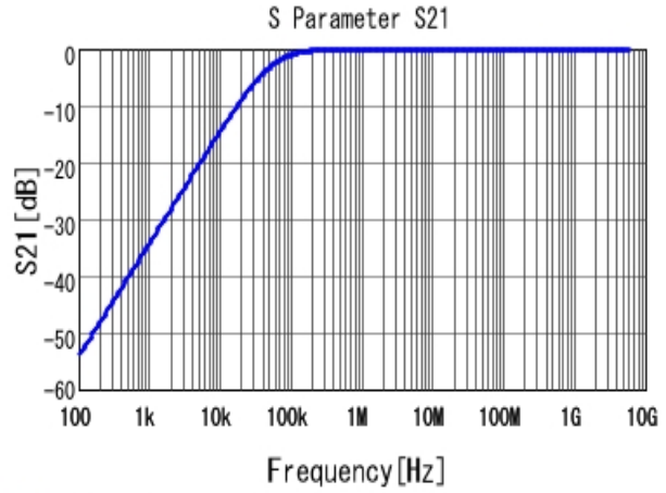
■ GRM155R71H333KE14 S21 DCOV, 25degC
