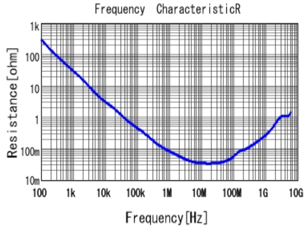
■ GRM155R71H333KE14 R DCOV, 25degC
