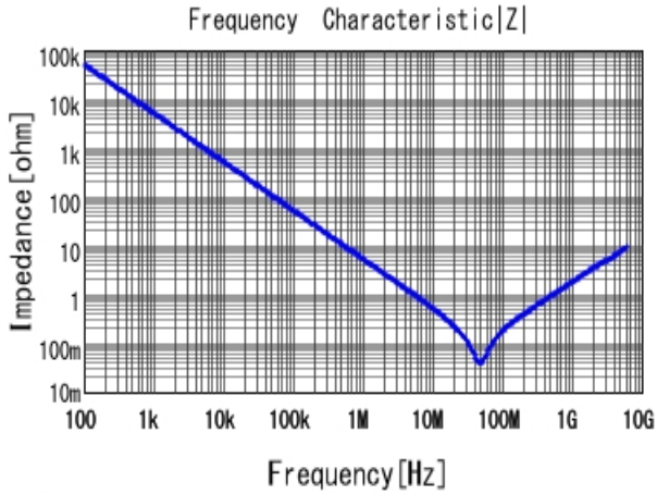
■ GRM155R71H333KE14 |Z| DCOV, 25degC
