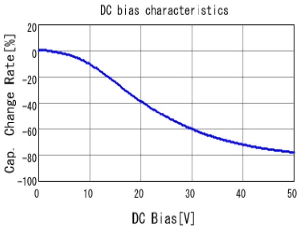
■ GRM155R71H333KE14 C-DC bias capchange, 25.0degC, AC1.
