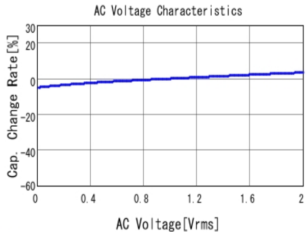
■ GRM155R71H333KE14 C-AC Voltage capchange, DCOV, 25.0d
