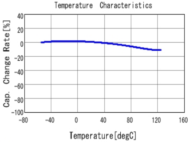
■ GRM155R71H333KE14 C-Temp. capchange, DCO. 0V, AC1.0V rm
