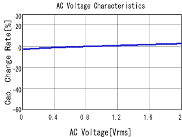
■ GRM155R71H332KA01 C-AC Voltage capchange, DC0V, 25.0d
