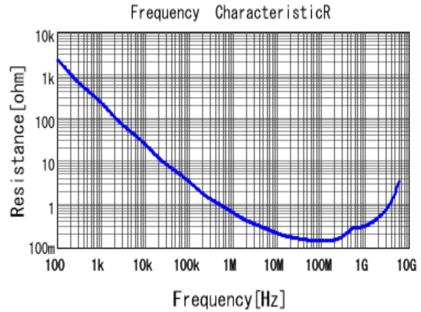
■ GRM155R71H332KA01 R DC0V, 25degC
