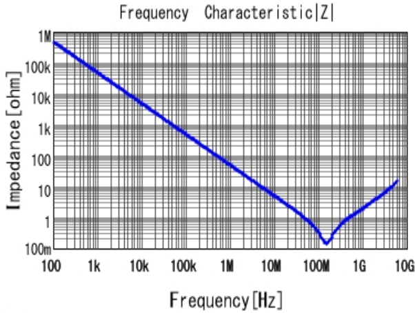
■ GRM155R71H332KA01 |Z| DC0V, 25degC
