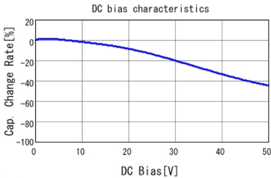
■ GRM155R71H272KA01 C-DC bias capchange, 25.0degC, AC1.
