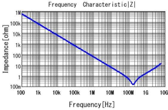
■ GRM155R71H272KA01 |Z| DCOV, 25degC
