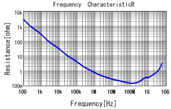
■ GRM155R71H272KA01 R DCOV, 25degC
