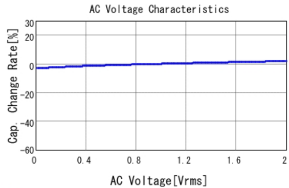
■ GRM155R71H272KA01 C-AC Voltage capchange, DCOV, 25.0d
