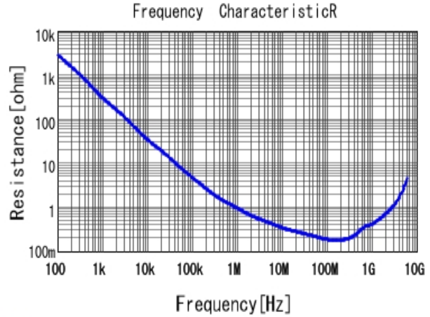
■ GRM155R71H222KA01 R DCOV, 25degC
