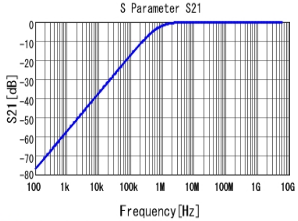
■ GRM155R71H222KA01 S21 DCOV, 25degC
