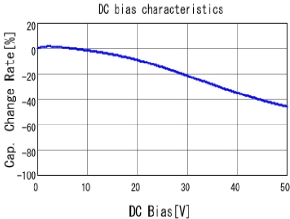
■ GRM155R71H222KA01 C-DC bias capchange, 25.0degC, AC1.
