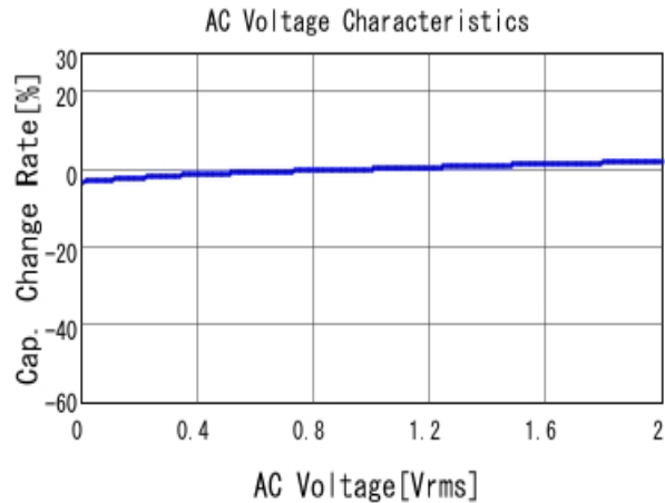
■ GRM155R71H222KA01 C-AC Voltage capchange, DCOV, 25.0d
