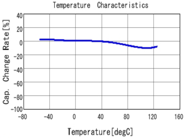
■ GRM155R71H222KA01 C-Temp. capchange, DCO. 0V, AC1.0Vrm
