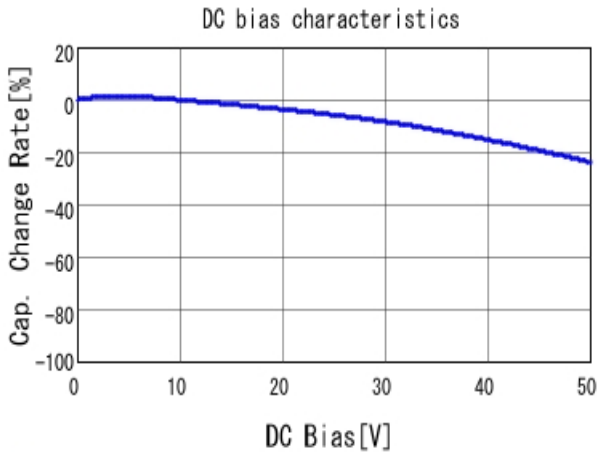
■ GRM155R71H221KA01 C-DC bias capchange, 25.0degC, AC1.
