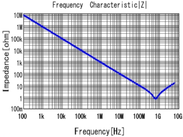
■ GRM155R71H221KA01 |Z| DCOV, 25degC
