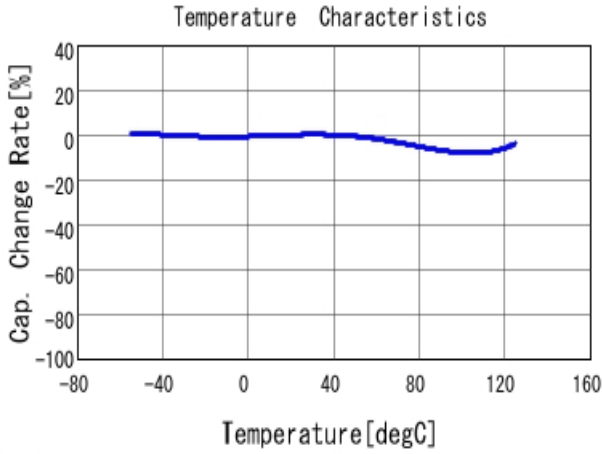
■ GRM155R71H221KA01 C-Temp. capchange, DCO. 0V, AC1.0Vrm
