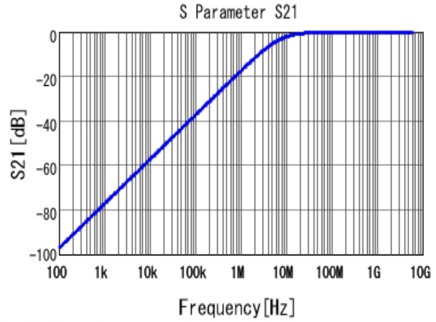
■ GRM155R71H221KA01 S21 DCOV, 25degC
