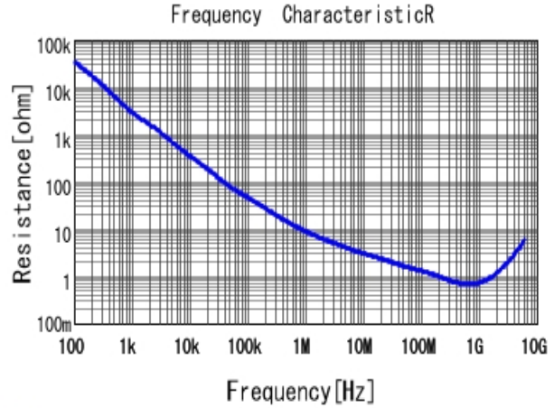
■ GRM155R71H221KA01 R DCOV, 25degC
