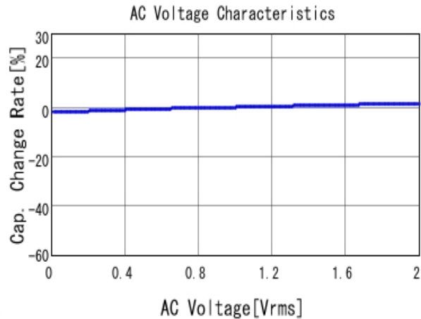
■ GRM155R71H221KA01 C-AC Voltage capchange, DCOV, 25.0d
