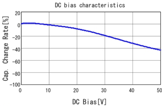
■ GRM155R71H182KA01 C-DC bias capchange, 25.0degC, AC1.
