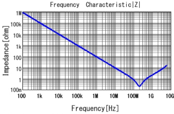
■ GRM155R71H182KA01 |Z| DCOV, 25degC
