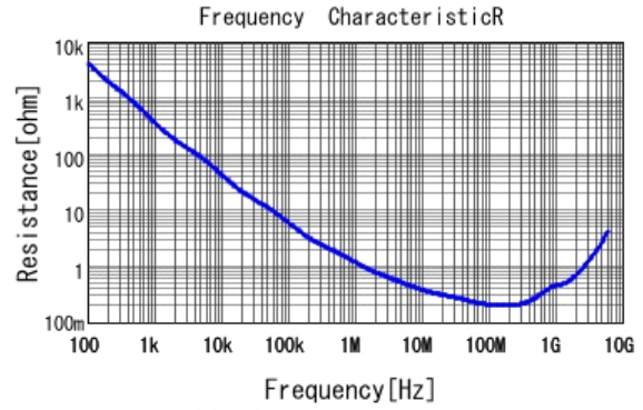
■ GRM155R71H182KA01 R DCOV, 25degC
