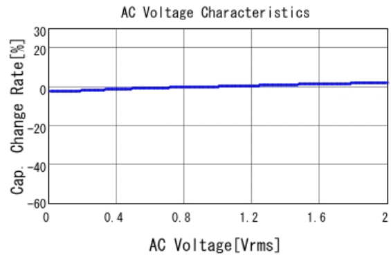
■ GRM155R71H182KA01 C-AC Voltage capchange, DCOV, 25.0d
