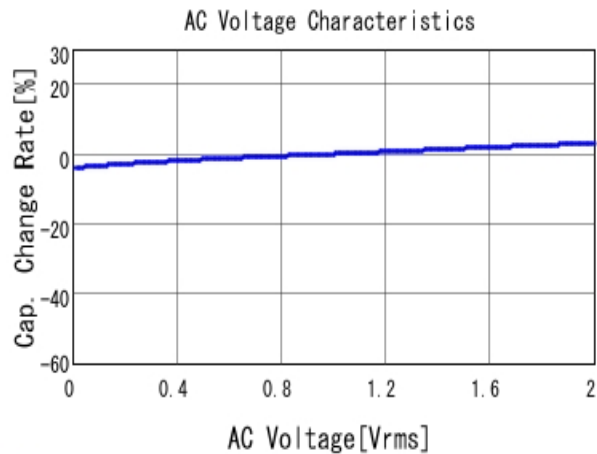
■ GRM155R71H153KA12 C-AC Voltage capchange, DCOV, 25.0d
