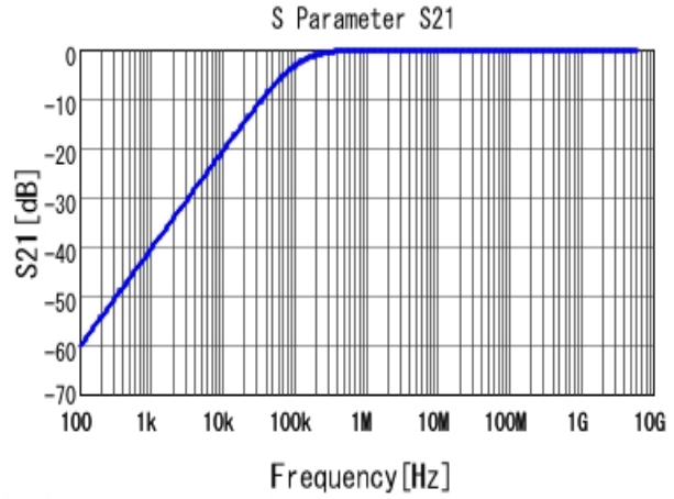
■ GRM155R71H153KA12 S21 DCOV, 25degC
