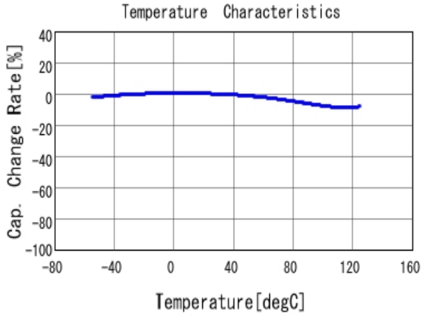
■ GRM155R71H153KA12 C-Temp. capchange, DCO. 0V, AC1.0Vrm
