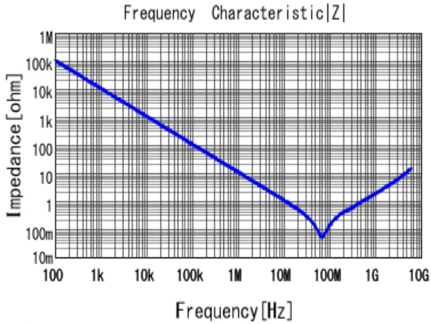
■ GRM155R71H153KA12 |Z| DCOV, 25degC
