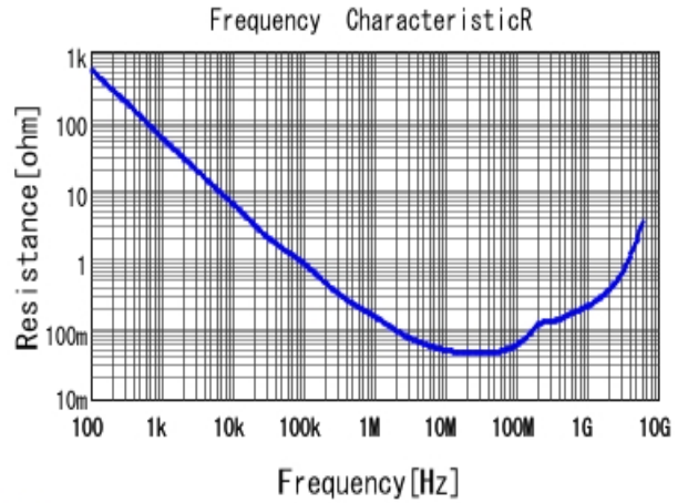
■ GRM155R71H153KA12 R DCOV, 25degC
