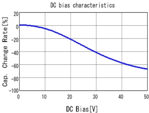
■ GRM155R71H153KA12 C-DC bias capchange, 25.0degC, AC1.
