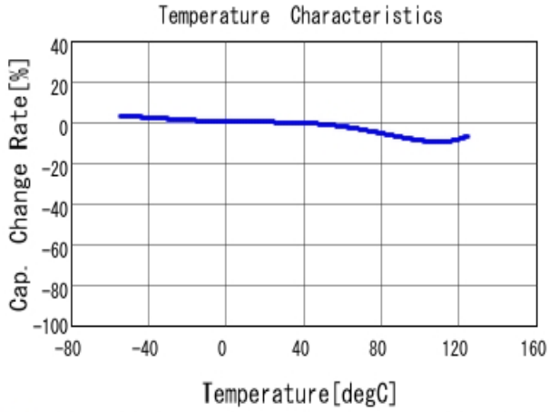
■ GRM155R71H152KA01 C-Temp. capchange, DCO. 0V, AC1.0Vrm
