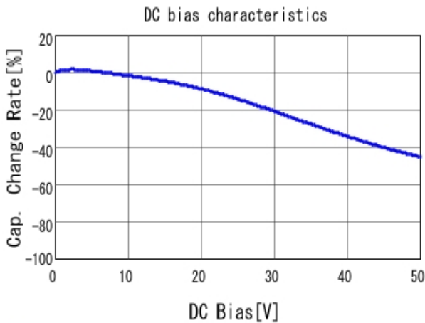
■ GRM155R71H152KA01 C-DC bias capchange, 25.0degC, AC1.
