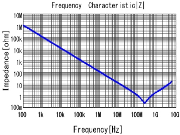
■ GRM155R71H152KA01 |Z| DCOV, 25degC
