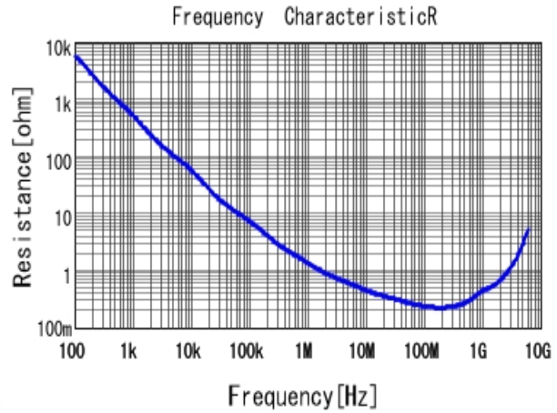
■ GRM155R71H152KA01 R DCOV, 25degC
