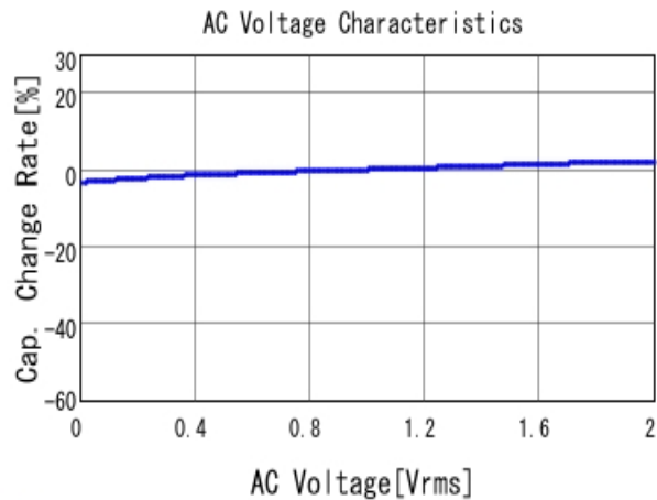
■ GRM155R71H152KA01 C-AC Voltage capchange, DCOV, 25.0d
