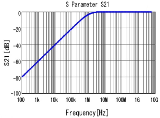
■ GRM155R71H152KA01 S21 DCOV, 25degC
