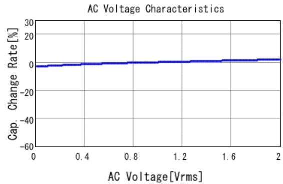
■ GRM155R71H122KA01 C-AC Voltage capchange, DCOV, 25.0d
