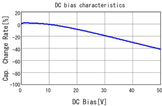
■ GRM155R71H122KA01 C-DC bias capchange, 25.0degC, AC1.
