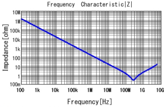
■ GRM155R71H122KA01 |Z| DCOV, 25degC
