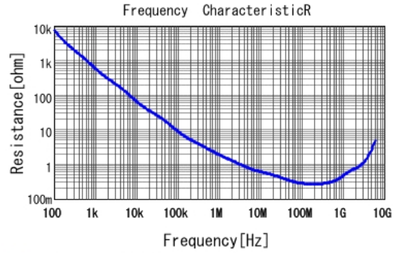
■ GRM155R71H122KA01 R DCOV, 25degC
