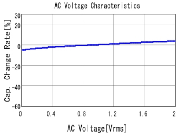
■ GRM155R71H104KE14 C-AC Voltage capchange, DCOV, 25.0d
