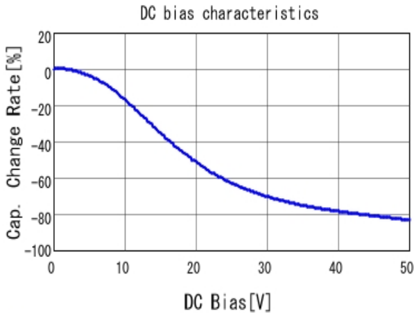
■ GRM155R71H104KE14 C-DC bias capchange, 25.0degC, AC1.
