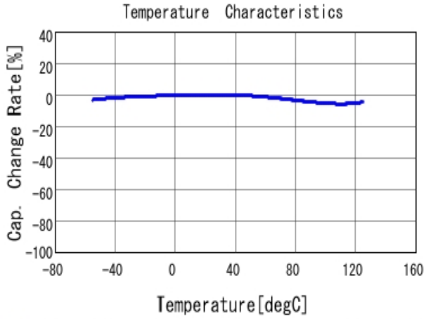
■ GRM155R71H103KA88 C-Temp. capchange, DCO. 0V, AC1.0V rm
