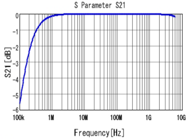
■ GRM155R71H103KA88 S21 DCOV, 25degC
