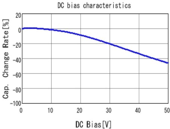
■ GRM155R71H103KA88 C-DC bias capchange, 25.0degC, AC1.
