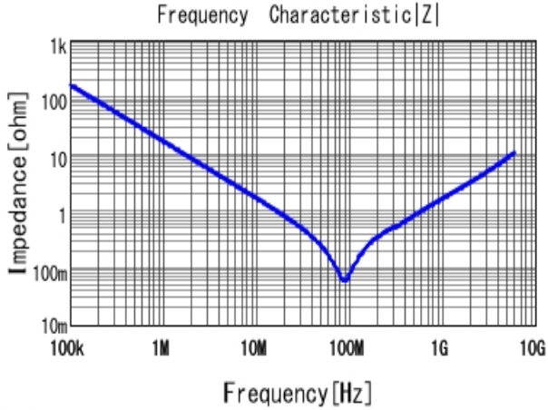
■ GRM155R71H103KA88 |Z| DCOV, 25degC
