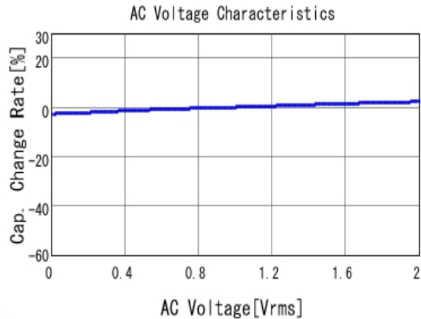
■ GRM155R71H103KA88 C-AC Voltage capchange, DCOV, 25.0d
