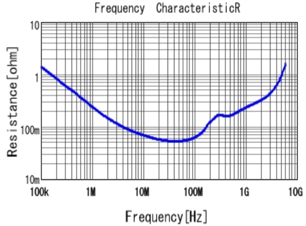
■ GRM155R71H103KA88 R DCOV, 25degC
