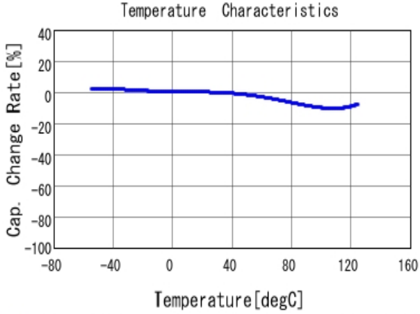
■ GRM155R71H102KA01 C-Temp. capchange, DCO. 0V, AC1.0V rm
