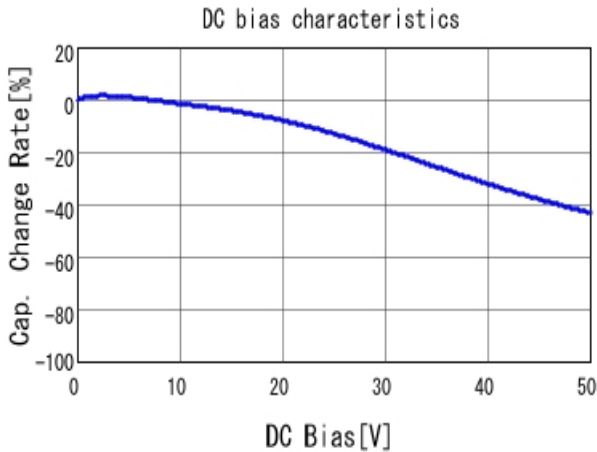
■ GRM155R71H102KA01 C-DC bias capchange, 25.0degC, AC1.
