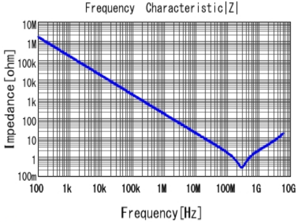
■ GRM155R71H102KA01 |Z| DCOV, 25degC
