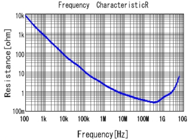
■ GRM155R71H102KA01 R DCOV, 25degC
