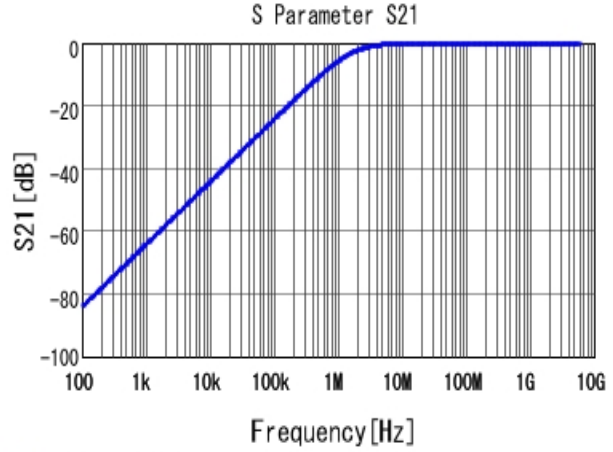
■ GRM155R71H102KA01 S21 DCOV, 25degC
