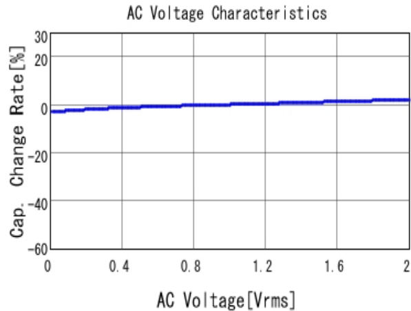
■ GRM155R71H102KA01 C-AC Voltage capchange, DCOV, 25.0d
