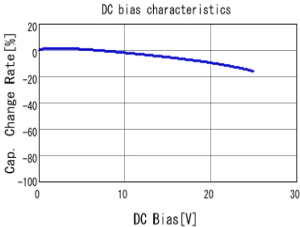
■ GRM155R71E472KA01 C-DC bias capchange, 25.0degC, AC1.
