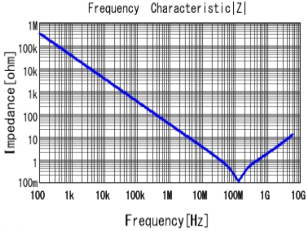
■ GRM155R71E472KA01 |Z| DCOV, 25degC
