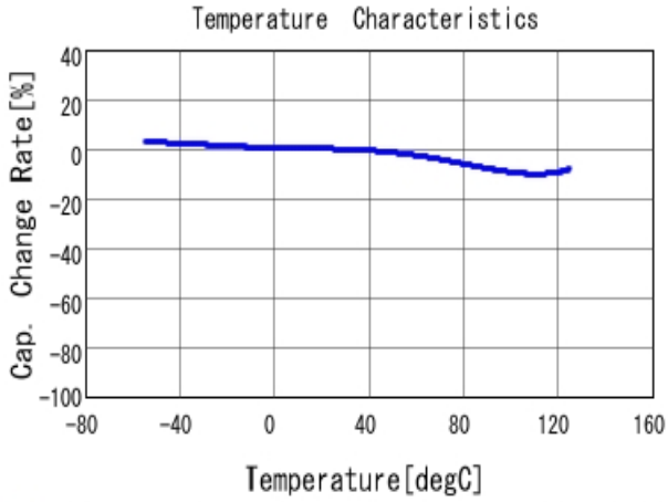
■ GRM155R71E472KA01 C-Temp. capchange, DCO. 0V, AC1.0Vrm
