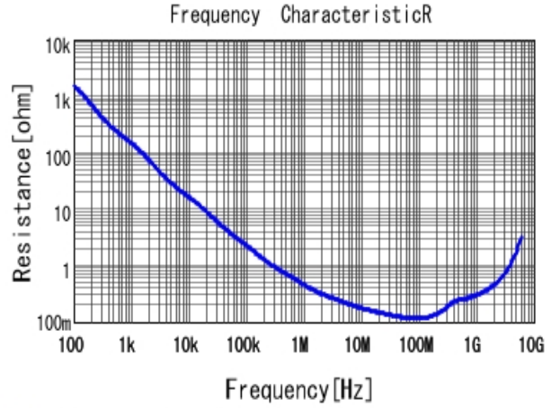
■ GRM155R71E472KA01 R DCOV, 25degC
