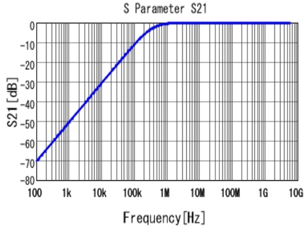
■ GRM155R71E472KA01 S21 DCOV, 25degC
