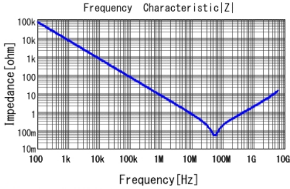
■ GRM155R71E223KA61 |Z| DCOV, 25degC
