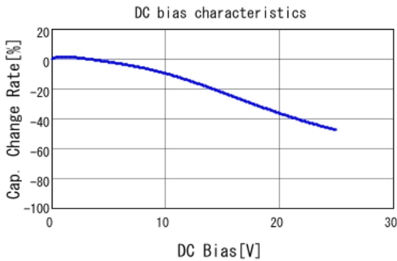
■ GRM155R71E223KA61 C-DC bias capchange, 25.0degC, AC1.
