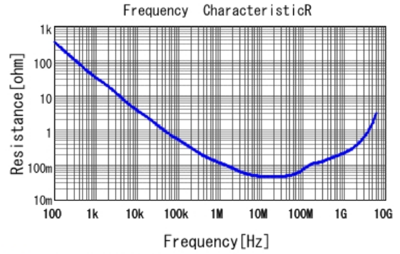
■ GRM155R71E223KA61 R DCOV, 25degC
