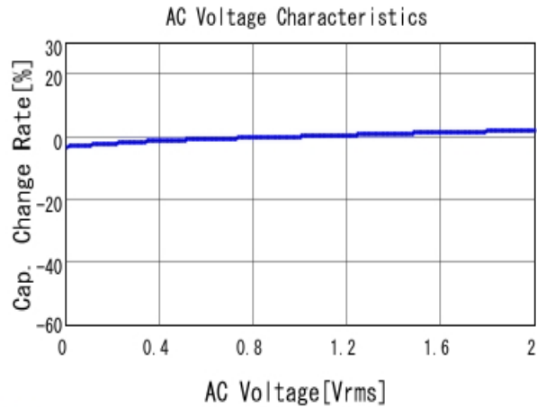
■ GRM155R71E222KA01 C-AC Voltage capchange, DCOV, 25.0d
