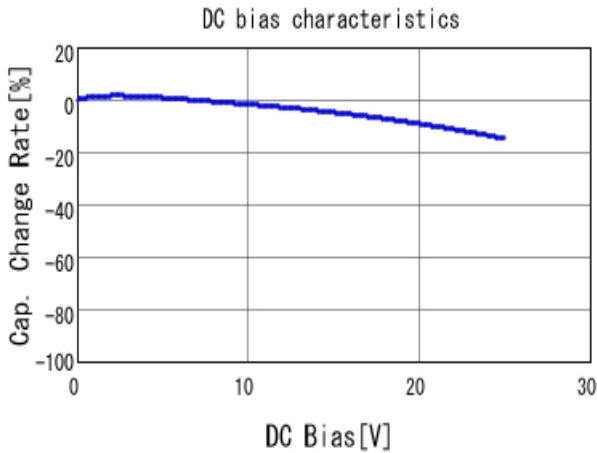
■ GRM155R71E222KA01 C-DC bias capchange, 25.0degC, AC1.
