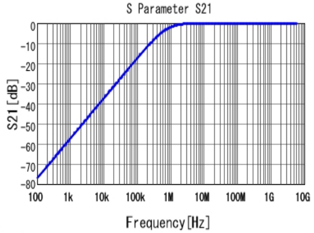
■ GRM155R71E222KA01 S21 DCOV, 25degC
