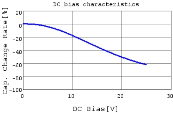
GRM155R71E104ME14 C-DC bias capchange, 25.0c
