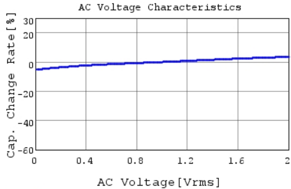
GRM155R71E104ME14 C-AC Voltage capchange, Dc
