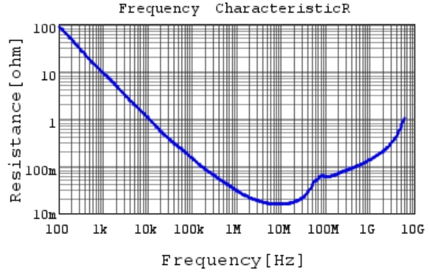
GRM155R71E104ME14 R DCOV, 25degC
