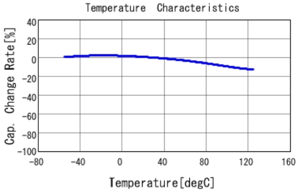
GRM155R71E104KE14 C-Temp. capchange, DC0.0V, AC1.C
