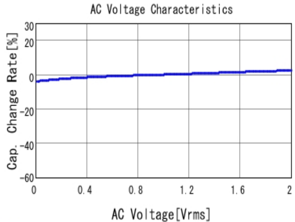
■ GRM155R71E103KA01 C-AC Voltage capchange, DCOV, 25.0d
