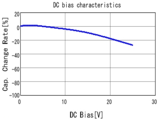
■ GRM155R71E103KA01 C-DC bias capchange, 25.0degC, AC1.
