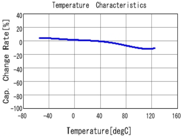
■ GRM155R71E103KA01 C-Temp. capchange, DCO. 0V, AC1.0Vrm
