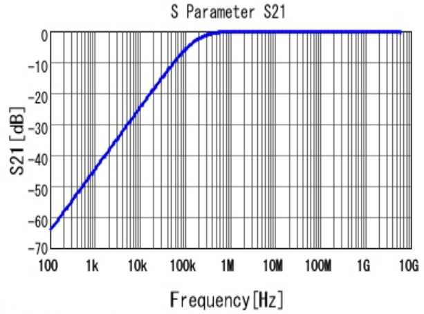
■ GRM155R71E103KA01 S21 DCOV, 25degC
