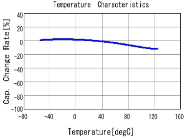
■ GRM155R71C683KA88 C-Temp. capchange, DCO. 0V, AC1.0V rm
