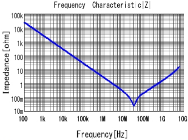
■ GRM155R71C683KA88 |Z| DCOV, 25degC
