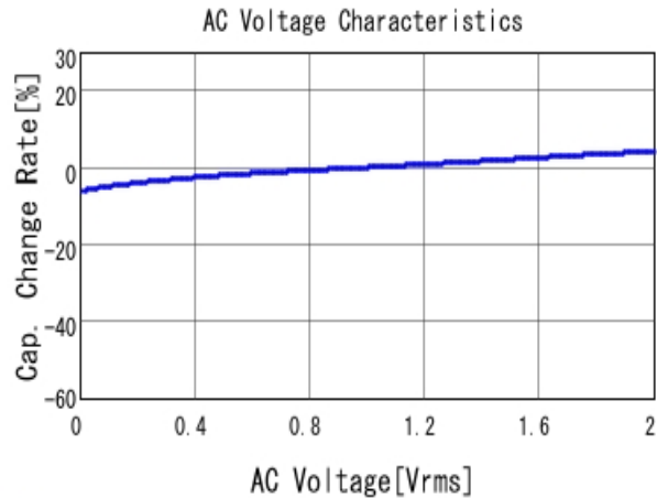
■ GRM155R71C683KA88 C-AC Voltage capchange, DCOV, 25.0d
