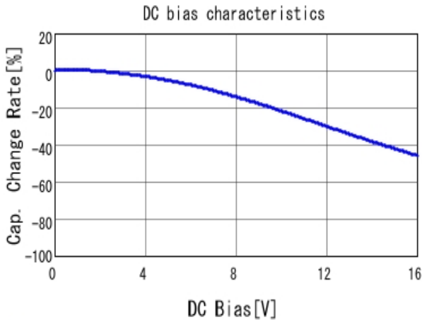
■ GRM155R71C683KA88 C-DC bias capchange, 25.0degC, AC1.
