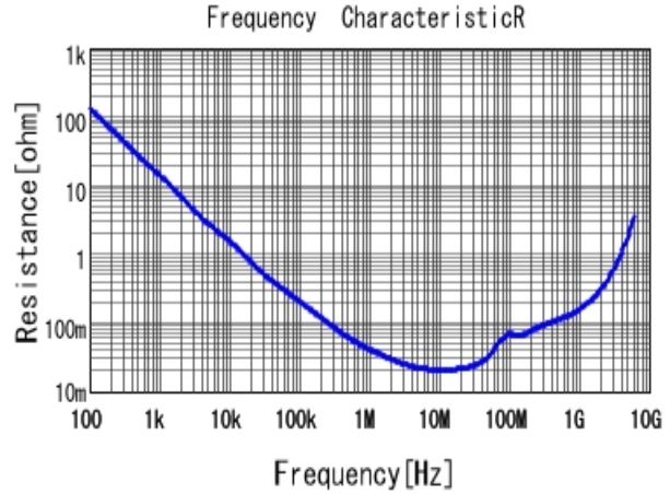
■ GRM155R71C683KA88 R DCOV, 25degC
