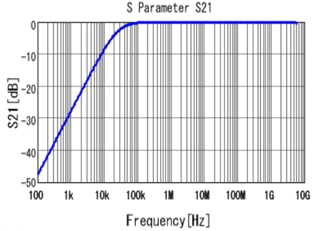
■ GRM155R71C683KA88 S21 DCOV, 25degC
