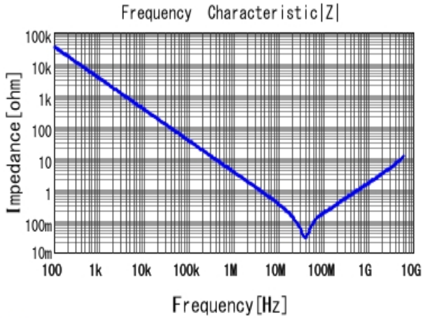
■ GRM155R71C473KA01 |Z| DCOV, 25degC
