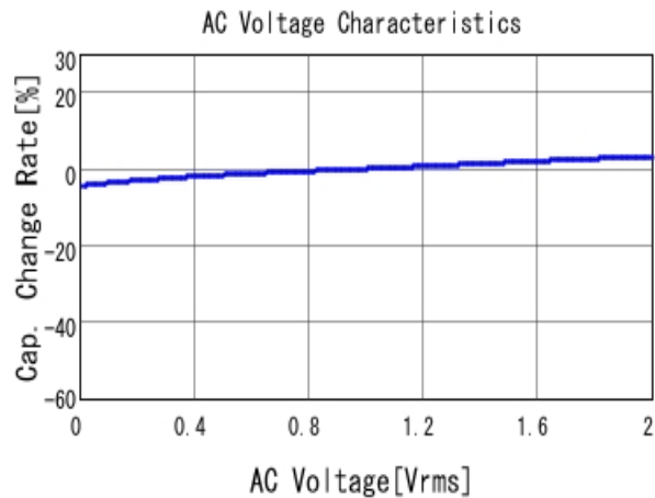
■ GRM155R71C473KA01 C-AC Voltage capchange, DCOV, 25.0d
