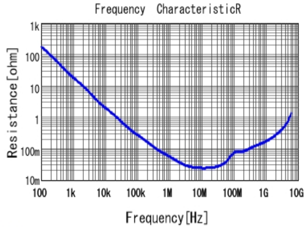
■ GRM155R71C473KA01 R DCOV, 25degC
