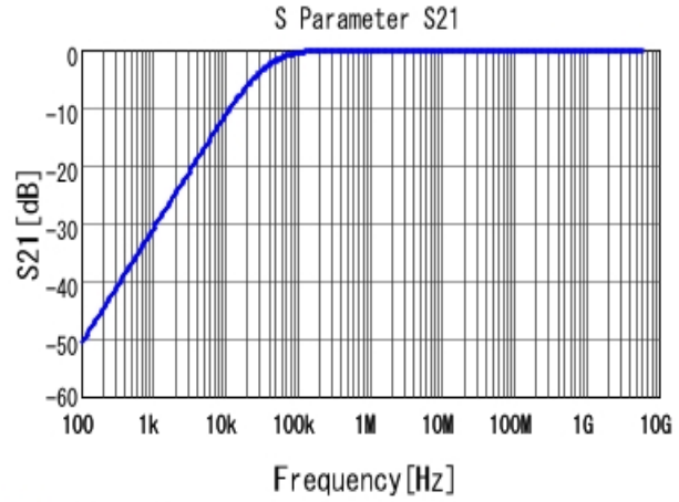
■ GRM155R71C473KA01 S21 DCOV, 25degC
