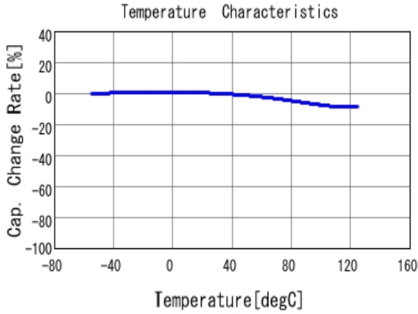
■ GRM155R71C473KA01 C-Temp. capchange, DCO. 0V, AC1.0Vrm
