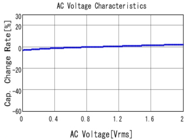
■ GRM155R71C472KA01 C-AC Voltage capchange, DCOV, 25.0d
