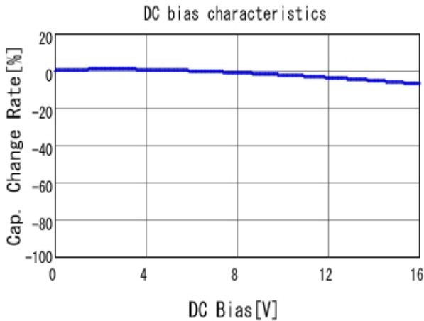
■ GRM155R71C472KA01 C-DC bias capchange, 25.0degC, AC1.
