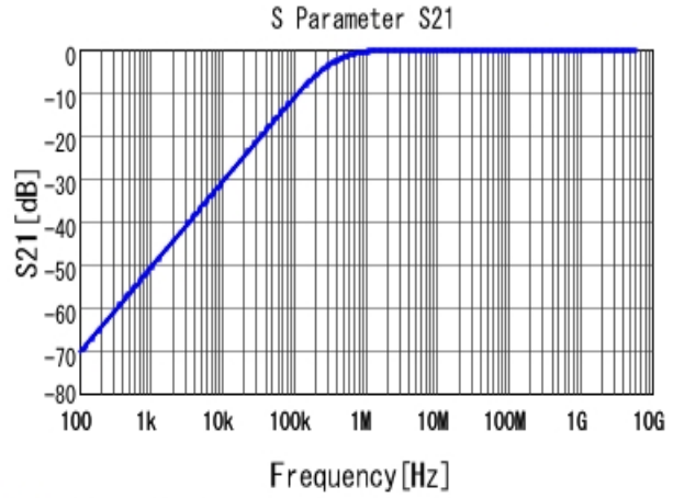
■ GRM155R71C472KA01 S21 DCOV, 25degC
