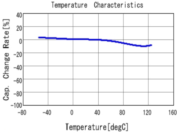
■ GRM155R71C472KA01 C-Temp. capchange, DCO. 0V, AC1.0Vrm
