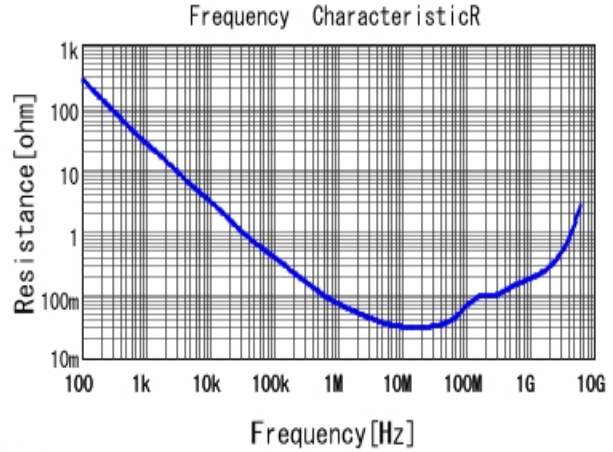
■ GRM155R71C333KA01 R DCOV, 25degC
