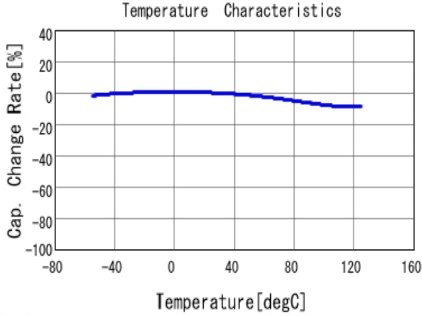
■ GRM155R71C333KA01 C-Temp. capchange, DCO. 0V, AC1.0V rm
