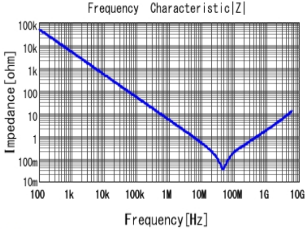
■ GRM155R71C333KA01 |Z| DCOV, 25degC
