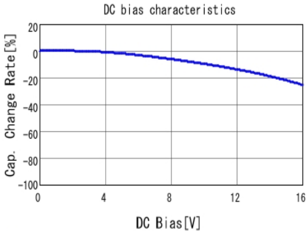
■ GRM155R71C333KA01 C-DC bias capchange, 25.0degC, AC1.
