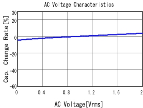
■ GRM155R71C333KA01 C-AC Voltage capchange, DCOV, 25.0d
