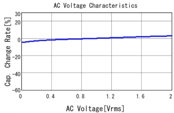
■ GRM155R71C223KA01 C-AC Voltage capchange, DCOV, 25.0d
