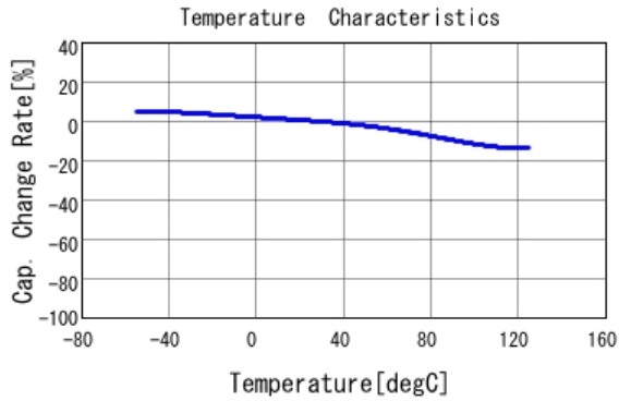
■ GRM155R71C223KA01 C-Temp. capchange, DC0.0V, AC1.0V rm
