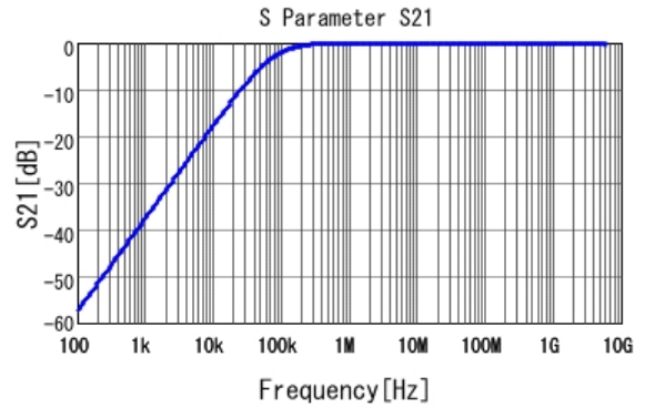
■ GRM155R71C223KA01 S21 DC0V, 25degC
