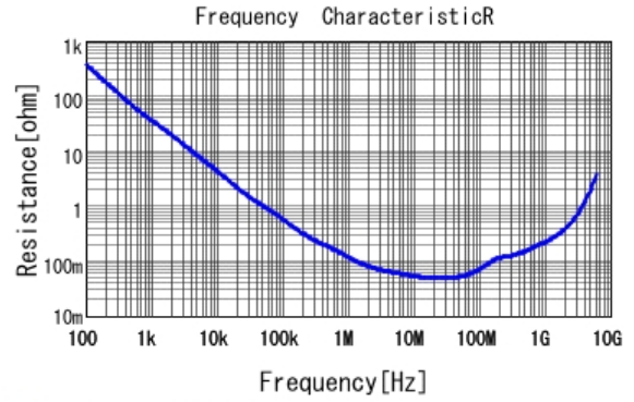
■ GRM155R71C223KA01 R DCOV, 25degC
