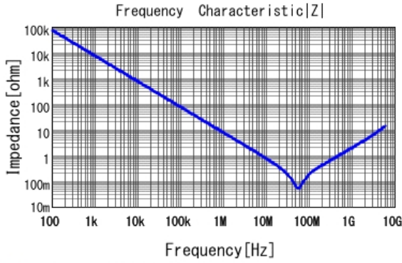
■ GRM155R71C223KA01 |Z| DCOV, 25degC
