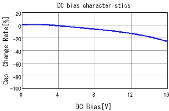
■ GRM155R71C223KA01 C-DC bias capchange, 25.0degC, AC1.
