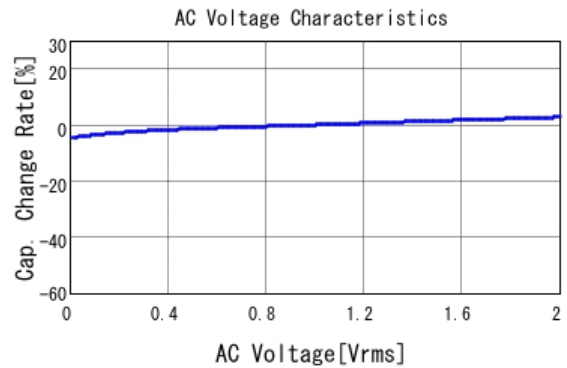
■ GRM155R71C183KA01 C-AC Voltage capchange, DCOV, 25.0d
