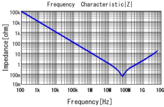
■ GRM155R71C183KA01 |Z| DCOV, 25degC
