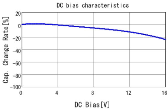
■ GRM155R71C183KA01 C-DC bias capchange, 25.0degC, AC1.
