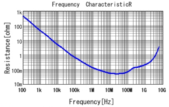
■ GRM155R71C183KA01 R DCOV, 25degC
