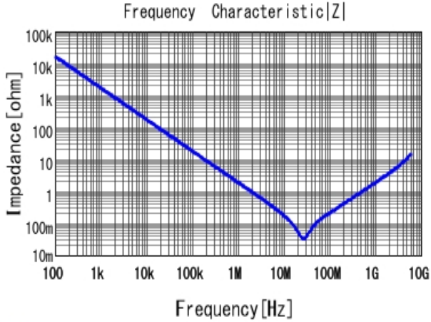
■ GRM155R71C154KA12 |Z| DCOV, 25degC
