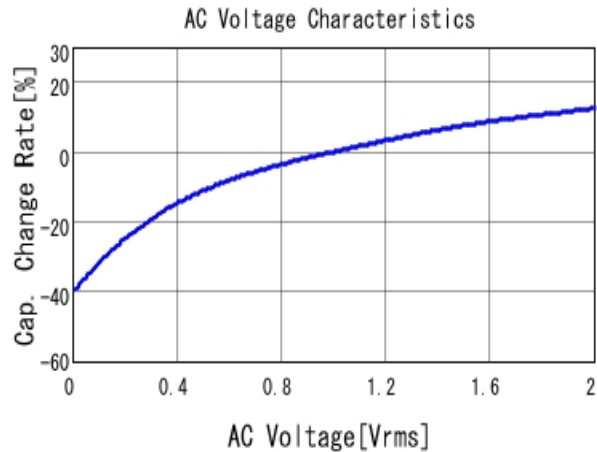
■ GRM155R71C154KA12 C-AC Voltage capchange, DCOV, 25.0d
