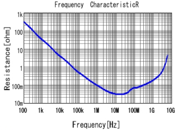
■ GRM155R71C154KA12 R DCOV, 25degC
