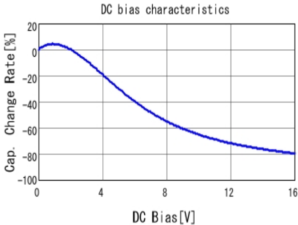
■ GRM155R71C154KA12 C-DC bias capchange, 25.0degC, AC1.
