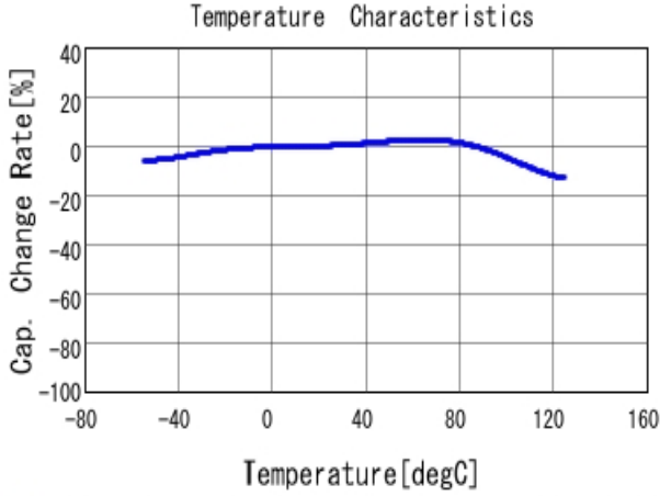
■ GRM155R71C154KA12 C-Temp. capchange, DC0.0V, AC1.0V rm
