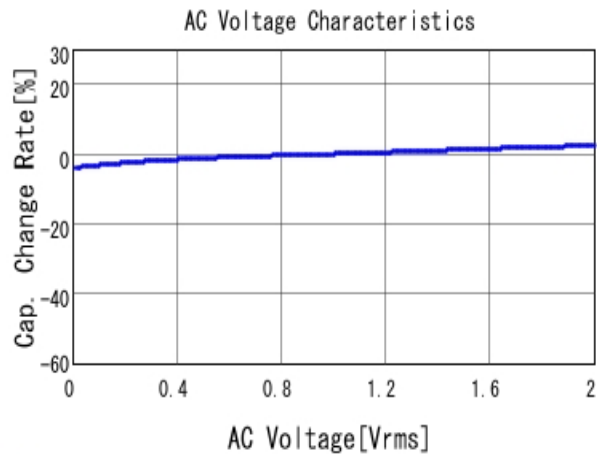
■ GRM155R71C103MA01 C-AC Voltage capchange, DCOV, 25.0d
