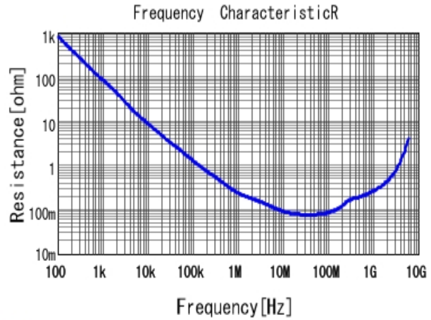
■ GRM155R71C103MA01 R DCOV, 25degC
