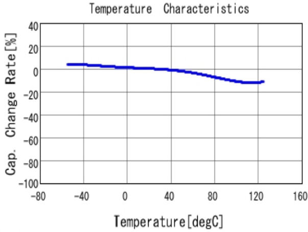
■ GRM155R71C103MA01 C-Temp. capchange, DCO. 0V, AC1.0V rm
