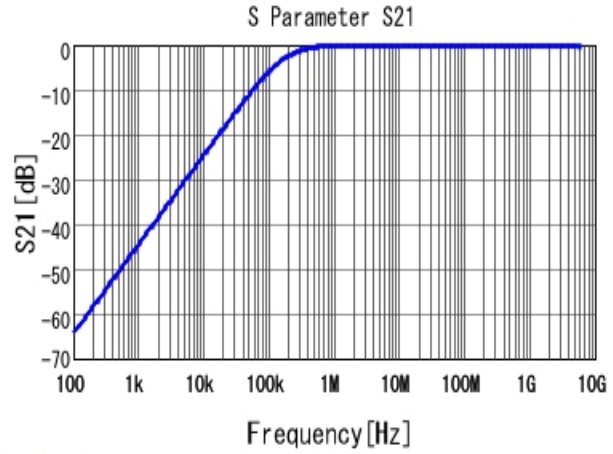
■ GRM155R71C103MA01 S21 DCOV, 25degC
