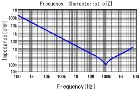
■ GRM155R71C103KA01 |Z| DCOV, 25degC
