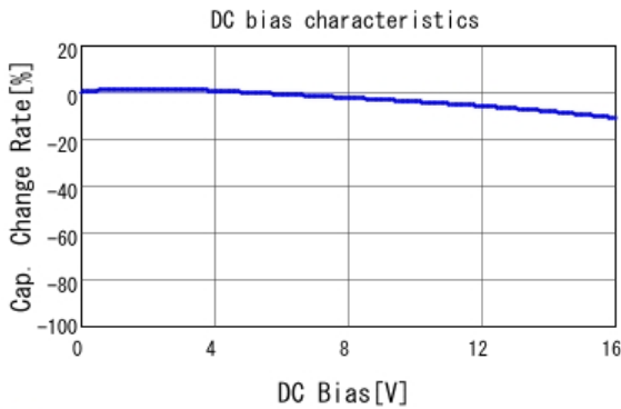
■ GRM155R71C103KA01 C-DC bias capchange, 25.0degC, AC1.
