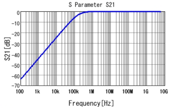
■ GRM155R71C103KA01 S21 DC0V, 25degC
