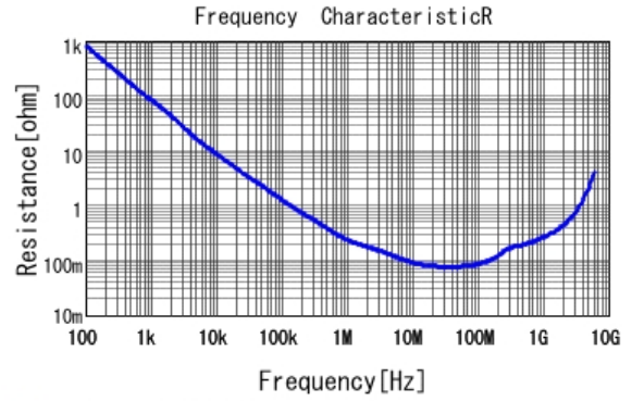
■ GRM155R71C103KA01 R DCOV, 25degC
