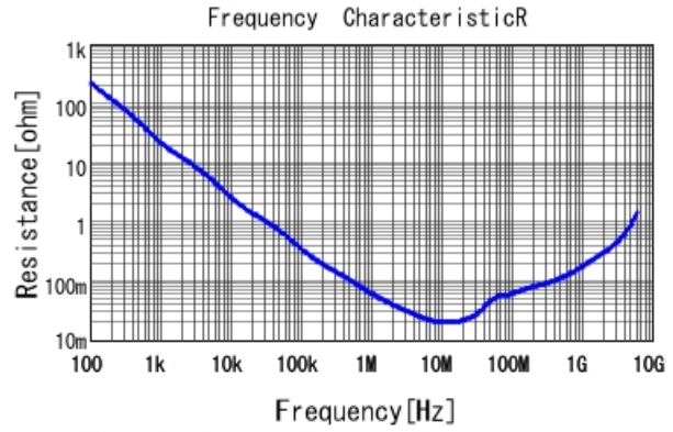
GRM155R71A224KE01 R DCOV, 25degC
