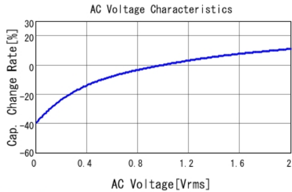
GRM155R71A224KE01 C-AC Voltage capchange, DCOV, 25
