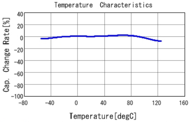
GRM155R71A224KE01 C-Temp. capchange, DC0.0V, AC1.C
