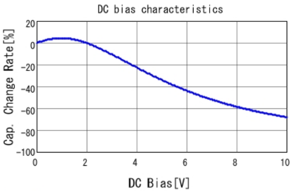
GRM155R71A224KE01 C-DC bias capchange, 25.0degC, A
