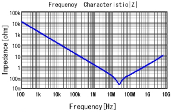
GRM155R71A224KE01 |Z| DCOV, 25degC
