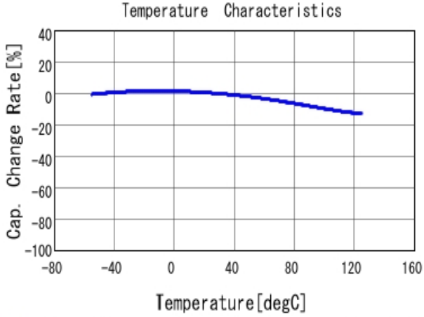
■ GRM155R71A104KA01 C-Temp. capchange, DC0.0V, AC1.0V rm
