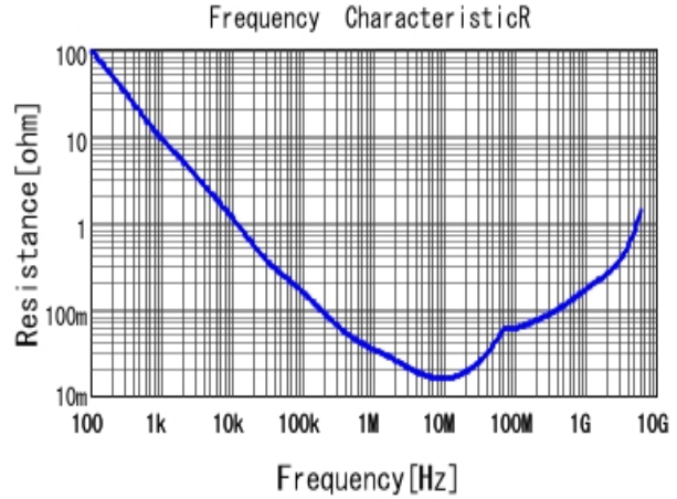
■ GRM155R71A104KA01 R DCOV, 25degC
