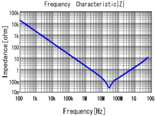
■ GRM155R71A104KA01 |Z| DCOV, 25degC
