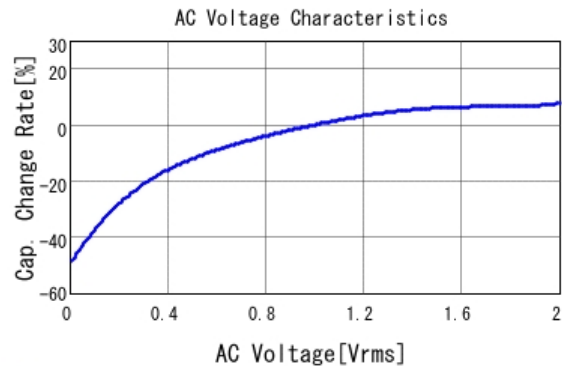
■ GRM155R70J105MA12 C-AC Voltage capchange, DCOV, 25.0d
