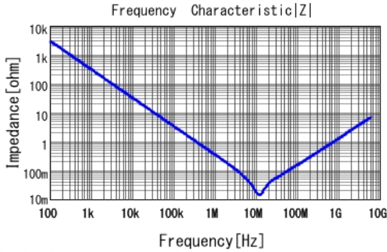
■ GRM155R70J105MA12 |Z| DCOV, 25degC
