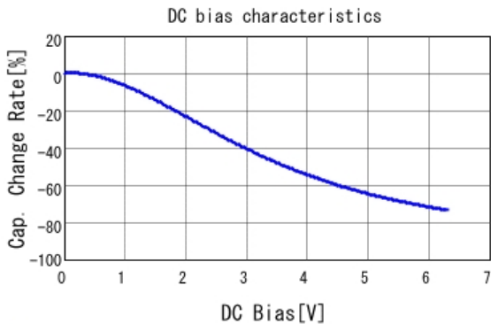
■ GRM155R70J105MA12 C-DC bias capchange, 25.0degC, AC1V
