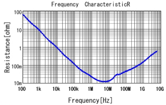
■ GRM155R70J105MA12 R DCOV, 25degC
