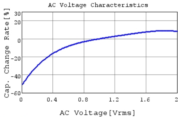
GRM155R70J105KA12 C-AC Voltage capchange, DC
