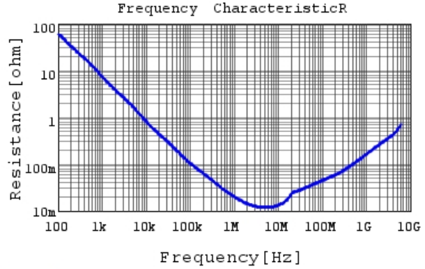
GRM155R70J105KA12 R DCOV, 25degC
