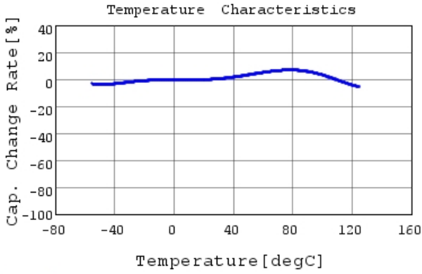
GRM155R70J105KA12 C-Temp. capchange, DC0.0V,
