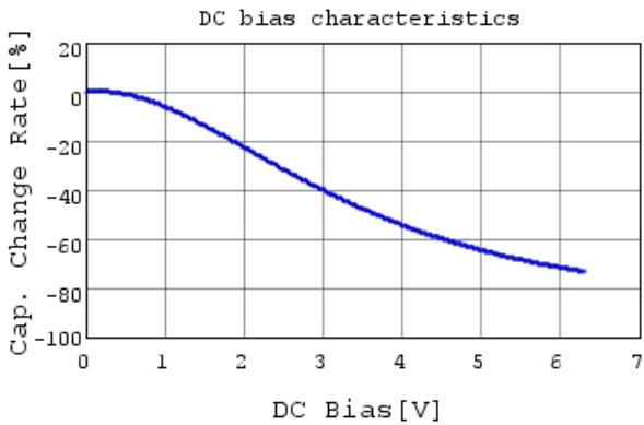
GRM155R70J105KA12 C-DC bias capchange, 25.0c
