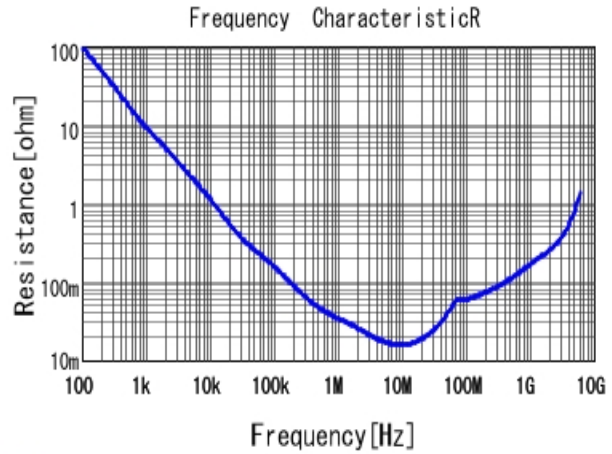
■ GRM155R70J104KA01 R DCOV, 25degC
