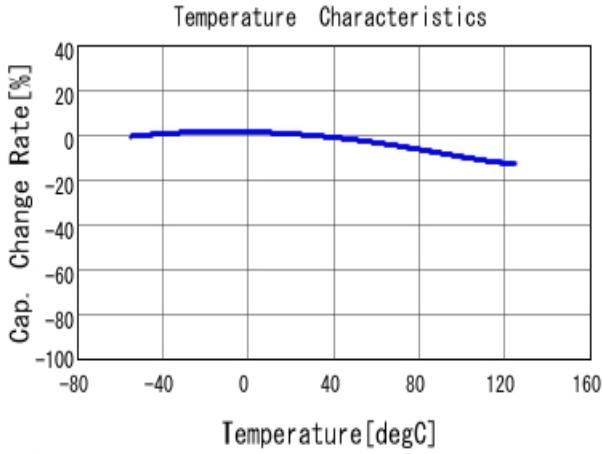
■ GRM155R70J104KA01 C-Temp. capchange, DC0.0V, AC1.0V r m
