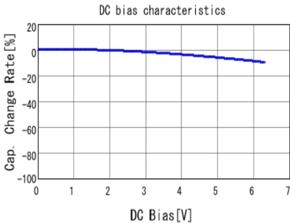
■ GRM155R70J104KA01 C-DC bias capchange, 25.0degC, AC1.
