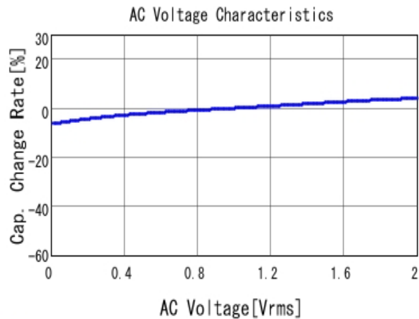
■ GRM155R70J104KA01 C-AC Voltage capchange, DCOV, 25.0d
