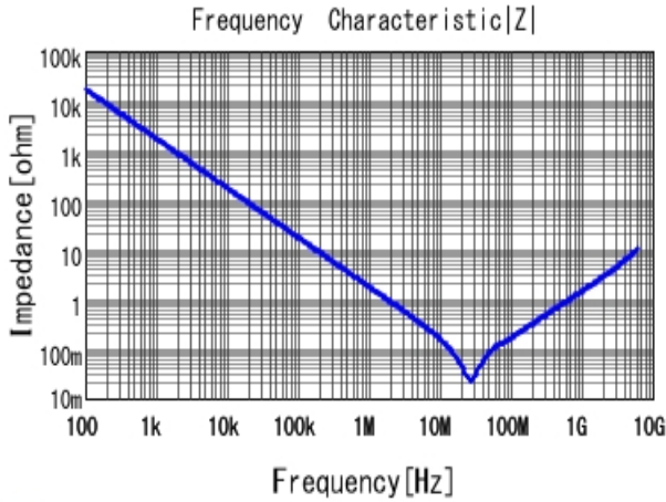
■ GRM155R70J104KA01 |Z| DCOV, 25degC
