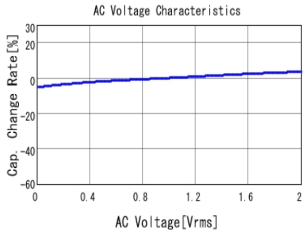
■ GRM155R62A104KE14 C-AC Voltage capchange, DCOV, 25.0d
