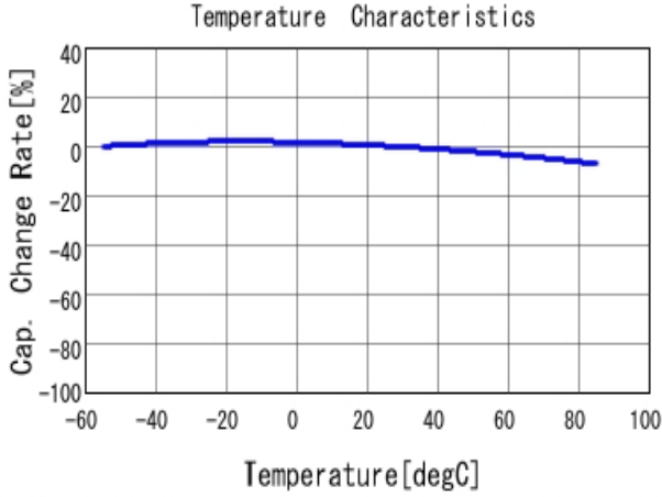
■ GRM155R62A104KE14 C-Temp. capchange, DC0.0V, AC1.0V rm
