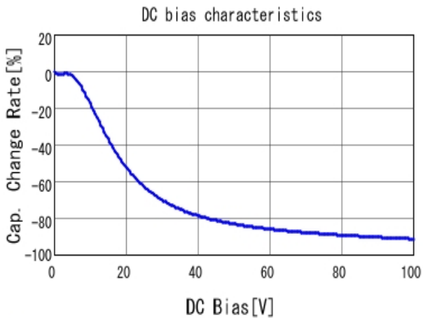
■ GRM155R62A104KE14 C-DC bias capchange, 25.0degC, AC1.
