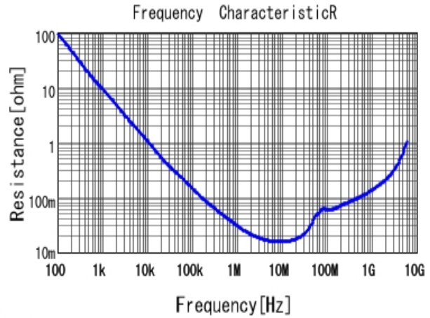
■ GRM155R62A104KE14 R DCOV, 25degC
