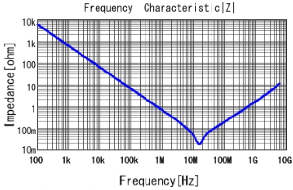
GRM155R61E474KE01 |Z| DCOV, 25degC
