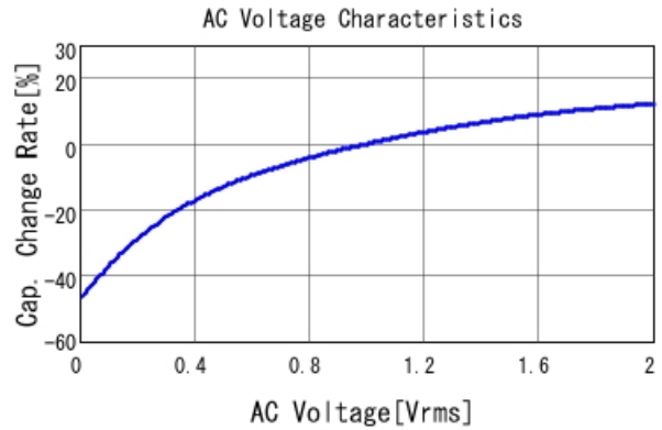
GRM155R61E474KE01 C-AC Voltage capchange, DCOV, 25
