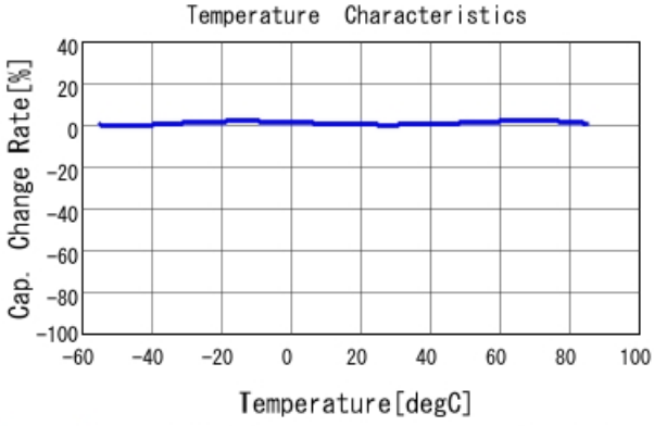
GRM155R61E474KE01 C-Temp. capchange, DC0.0V, AC1.C
