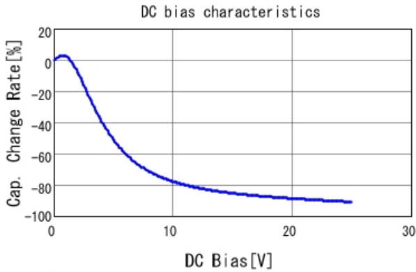
GRM155R61E474KE01 C-DC bias capchange, 25.0degC, A
