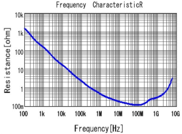
■ GRM155R61E472KA01 R DCOV, 25degC
