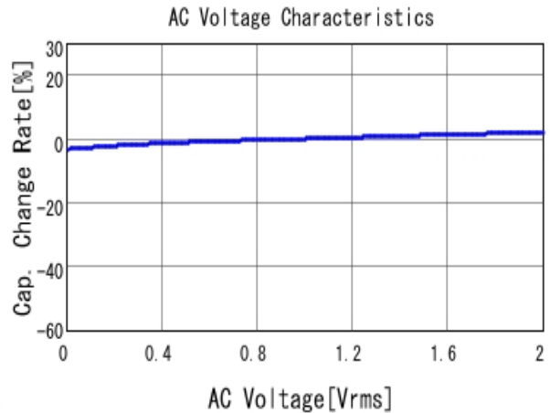
■ GRM155R61E472KA01 C-AC Voltage capchange, DCOV, 25.0d
