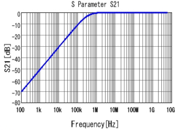
■ GRM155R61E472KA01 S21 DCOV, 25degC
