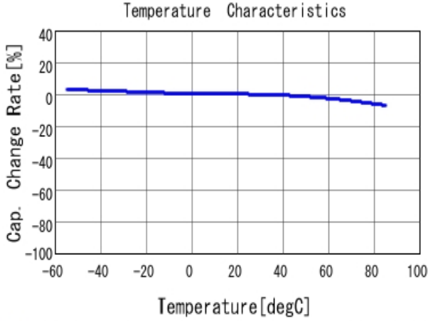
■ GRM155R61E472KA01 C-Temp. capchange, DCO. 0V, AC1.0V rm
