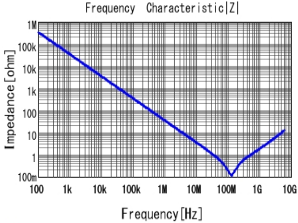
■ GRM155R61E472KA01 |Z| DCOV, 25degC
