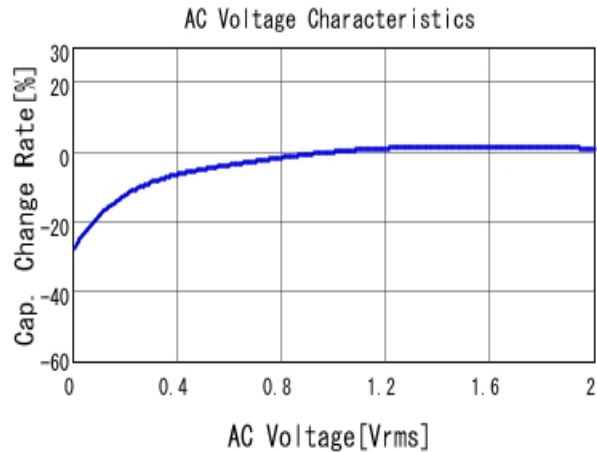
■ GRM155R61E225ME15 C-AC Voltage capchange, DCOV, 25.0d
