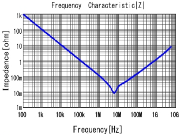
■ GRM155R61E225ME15 |Z| DCOV, 25degC
