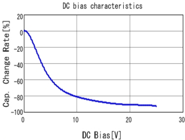
■ GRM155R61E225ME15 C-DC bias capchange, 25.0degC, AC1V
