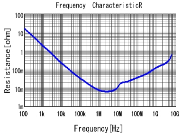
■ GRM155R61E225ME15 R DCOV, 25degC
